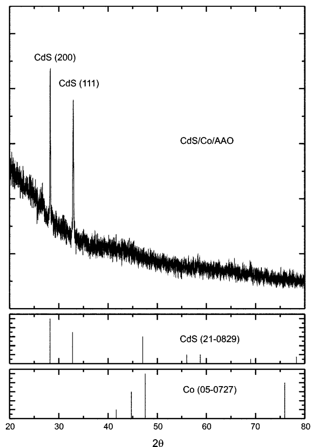
Figure 6. X-ray diffractogram of an as-deposited CdS/Co nanowire array in Figure 5. The vertical lines at the bottom of the figure indicate the standard position and relative intensities of hexagonal cadmium sulfide (ASTM 21-0829) and hexagonal cobalt (ASTM 05-0727), respectively.
