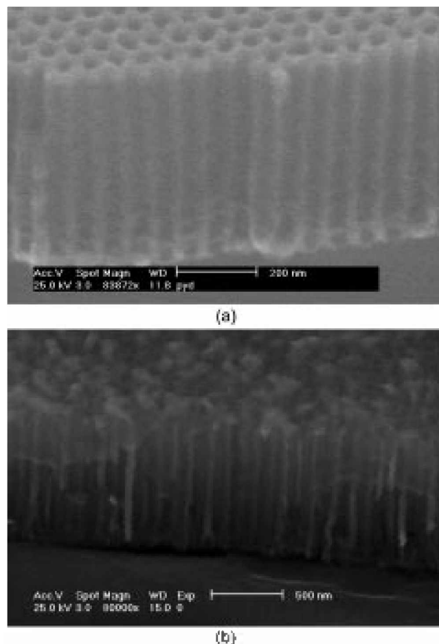
Figure 3. Prospective view SEM images of cobalt-filled AAO films underdeposited (a) and overdeposited (b).
