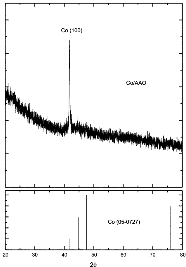
Figure 4. X-ray diffractogram of an as-deposited cobalt nanowire array in Figure 3b. The vertical lines at the bottom of the figure indicate the standard position and relative intensities of hexagonal cobalt (ASTM 05-0727).
