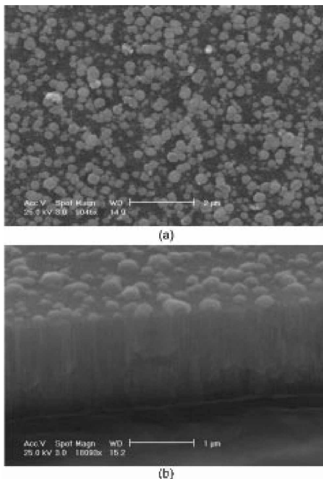
Figure 5. SEM images of a plan view (a) and a prospective view (b) of an CdS/Co nanowire array deposited in an AAO template.
