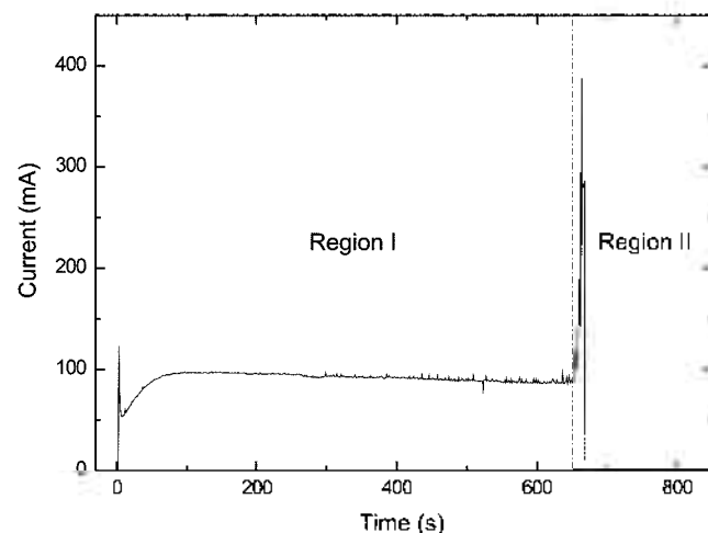
Figure 2. Current-time curve for electrodeposition of cobalt into an AAO film.
