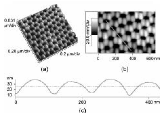
Figure 1. AFM images of 3-dimensional view (a), plan view (b) and height profile (c) of a pore morphology produced by anodizing aluminum.
