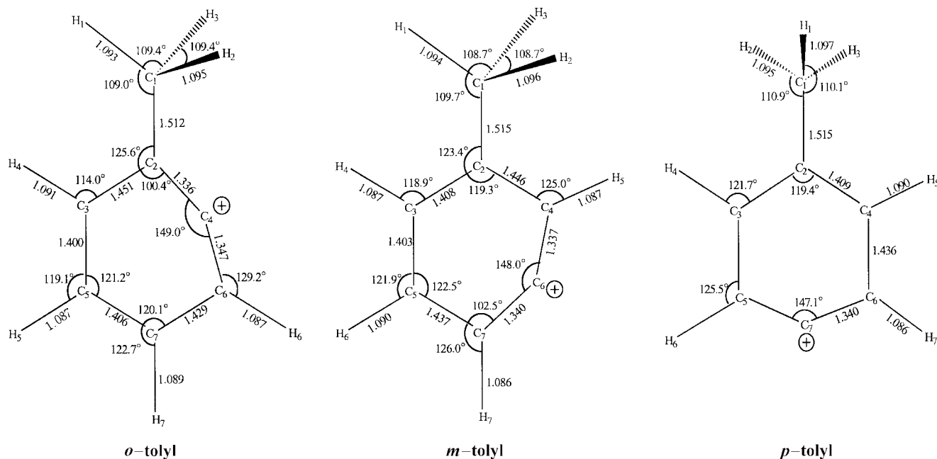
Figure 2. Predicted geometries for the o -, m -, and p -tolyl cations at the DZP CCSD level of theory. Bond lengths are in Å and bond angles are in degrees.
