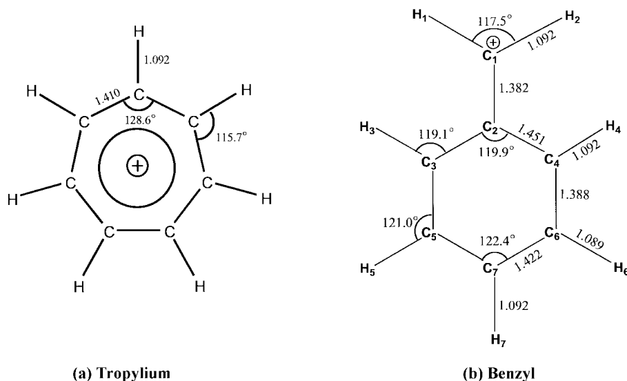
Figure 1. Predicted geometries for the (a) tropylium and (b) benzyl cations at the DZP CCSD(T) level of theory. Bond lengths are in Å and bond angles are in degrees.
