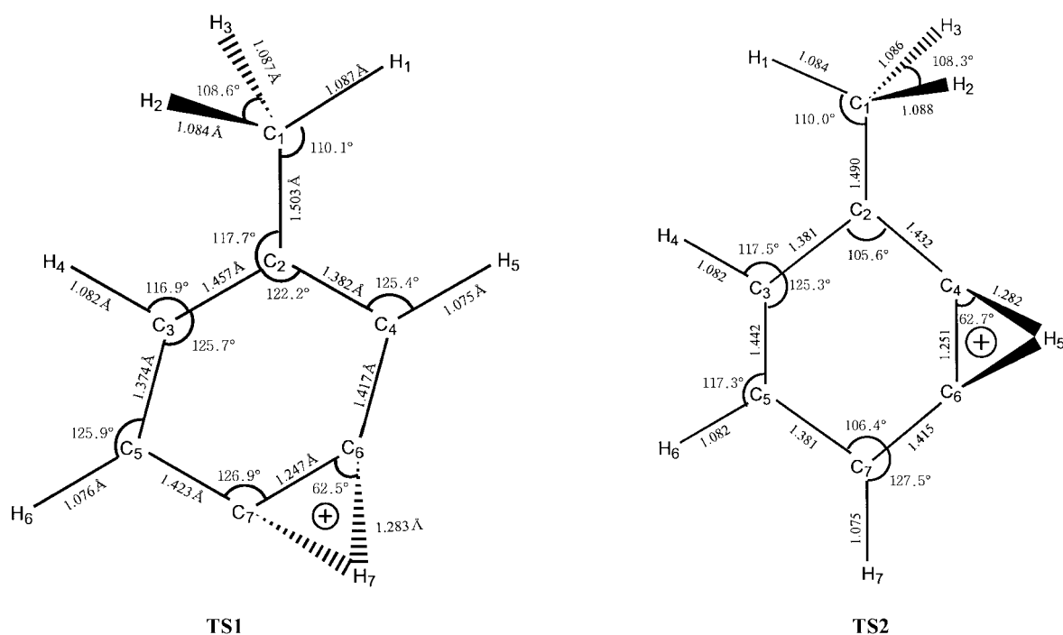
Figure 3. Predicted geometries for the transition states at the DZP CISD level of theory. TS1 is the transition state for the arrangement between the o - and the m -tolyl cations, and TS2 is the transition state for the arrangement between the m - and the p -tolyl cations. Bond lengths are in Å and bond angles are in degrees.
