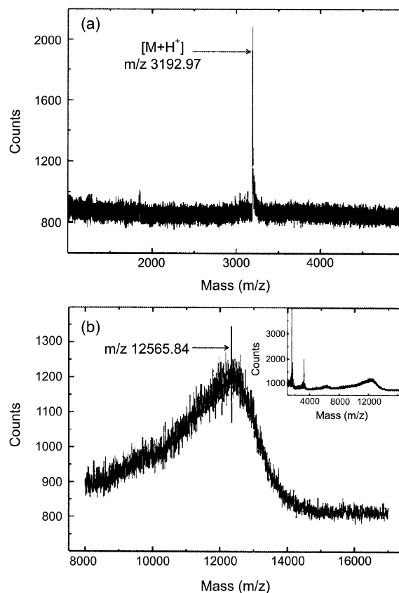
Figure 2. (a) MALDI-MS of PPI-Im 16 ; (b) MALDI-MS of PPI-Im 64 , the inset shows the full MS spectrum and fragmentation observed.
