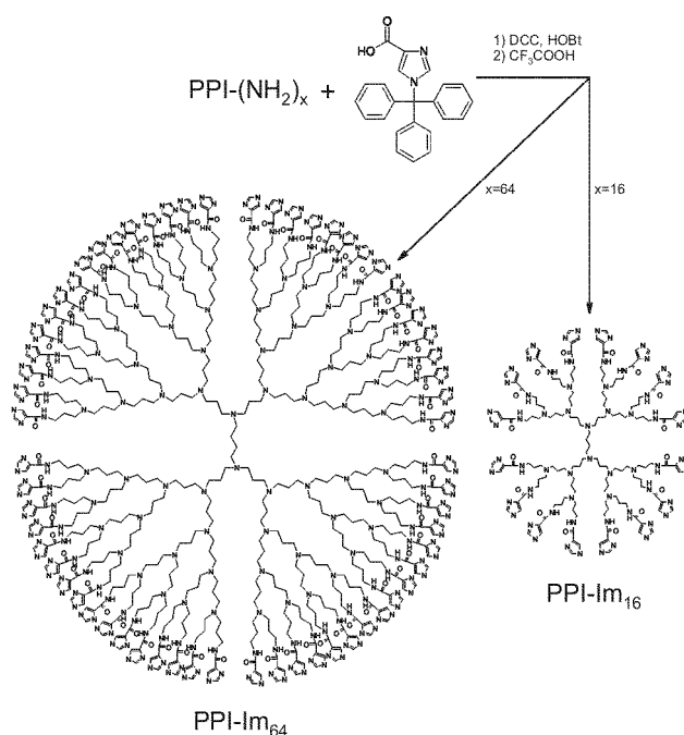
Figure 3. Synthesis of imidazole-terminated PPI dendrimers.
