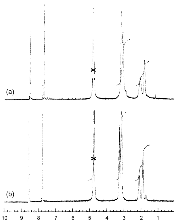
Figure 1. 1 H NMR (300 MHz) of (a) PPI-Im 64 and (b) PPI-Im 16 . (D 2 O/10% DCl)
