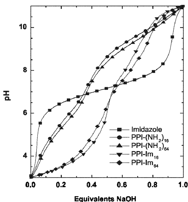
Figure 7. Titration (pH) of protonatable groups over the pH range 3-11.
