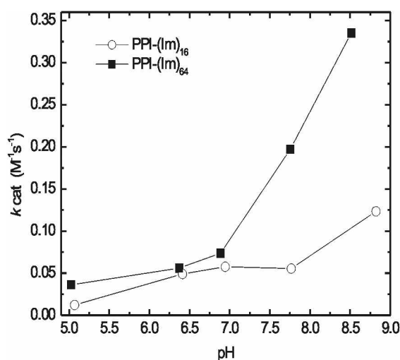
Figure 9. Catalysis ( k_{cat} ) of hydrolysis of 2,4-dinitrophenyl acetate as a function of pH for PPI-Im 16 and PPI-Im 64 .
