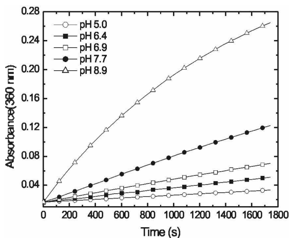
Figure 8. Measurement of hydrolysis of 2,4-dinitrophenyl acetate by PPI-Im 16 as a function of time and pH (uncorrected for background hydrolysis by buffer). [DNPA] = 2.5 \times 10^{-5} M, [PPI-Im 16 ] = 1.9 \times 10^{-5} M ([I] = 3.0 \times 10^{-1} M).
