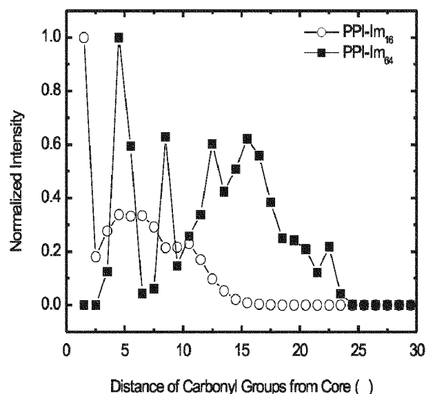
Figure 6. Measured distance of carbonyl groups from the core of the dendrimer.
