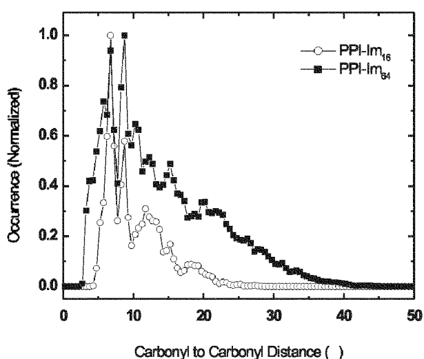
Figure 5. Measurement of carbonyl to carbonyl distance for PPI-Im 16 and PPI-Im 64 . Data are normalized to one at maximum.
