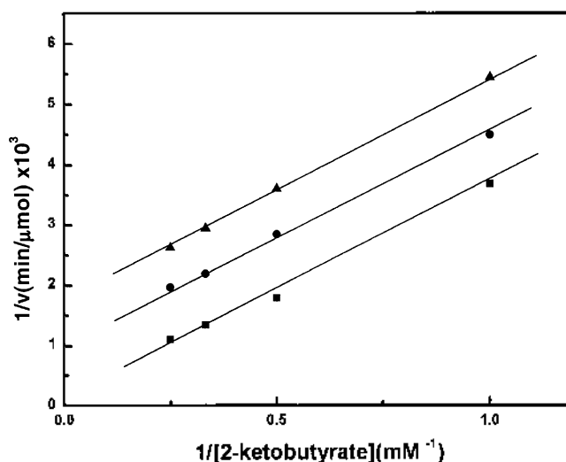
Figure 2. Dead-end inhibition pattern for the acetohydroxyacid synthase at pH 7.5. The assays were carried out under standard conditions. The 3-bromopyruvate concentrations were 0 mM (■), 2 mM (●) and 4 mM (▲) as a dead-end inhibitor of pyruvate. Points are experimental and the solid lines are from a fit using equation (3).
