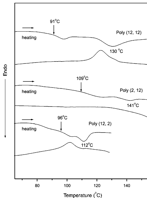
Figure 1. DSC thermograms of Poly (m, n)s.
