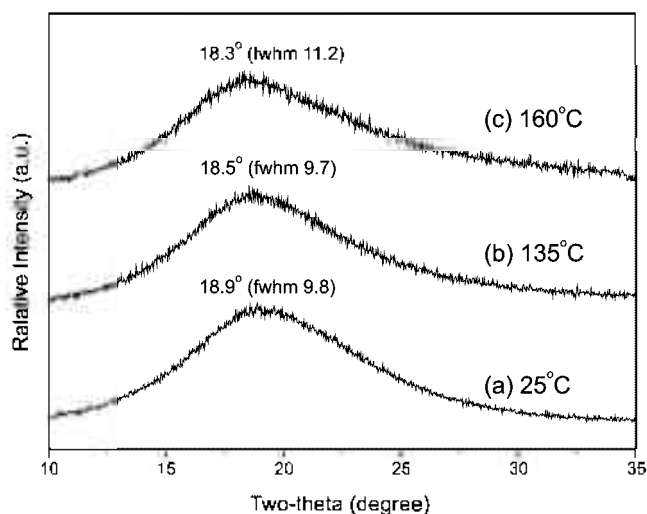
Figure 3. Wide-angle X-ray diffractograms of Poly (2, 12) at (a) 25 °C, (b) 135 °C, and (c) 160 °C.
