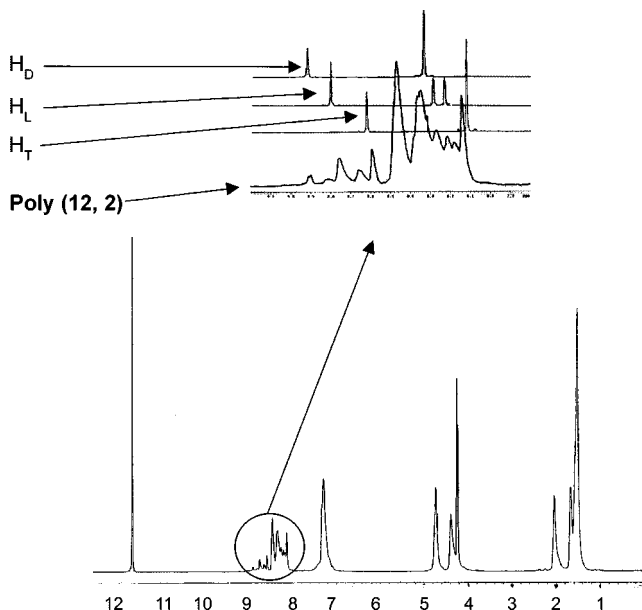
Figure 4. ^1\text{H-NMR} Spectra of Poly (12, 2) and their model compounds in \text{TFA-d} .
