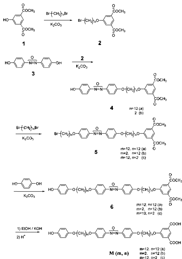
Scheme 1. Synthetic route to monomers.
