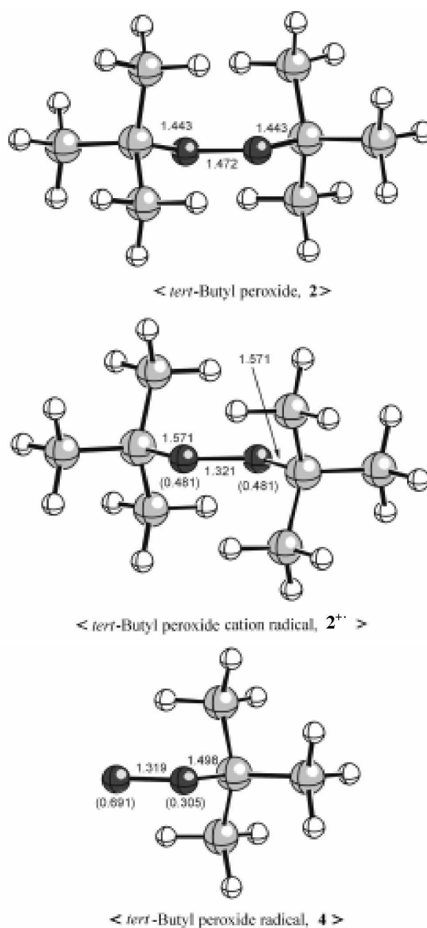
Figure 1. Optimized structures at UB3LYP/6-31G* level. Bond lengths are in Å and values in parentheses are spin densities in au.
