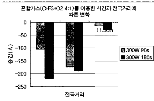
Fig. 11. A result of cleaning by plasma that add oxygen to CHF 3 under various operating conditions.
