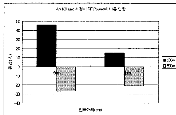
Fig. 3. A result of cleaning by argon plasma in various operating conditions.
