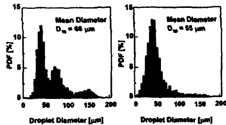
(a) Re_g = 4.14 \times 10^4 (b) Re_g = 8.28 \times 10^4
