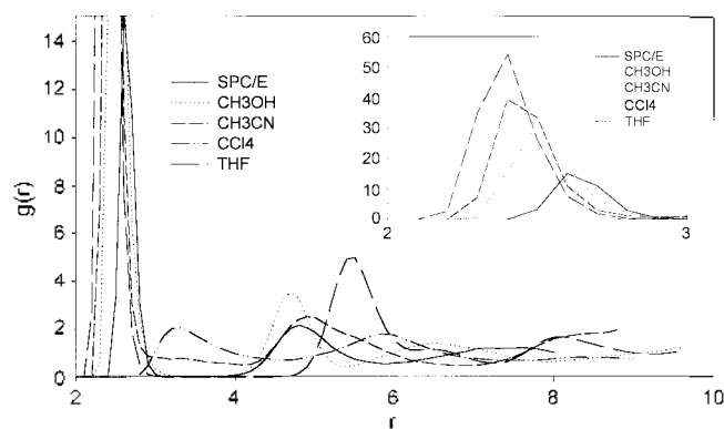
Figure 2. Radial distribution function of Eu 3+ ion in selected solvents. Distances are in angstroms throughout.
