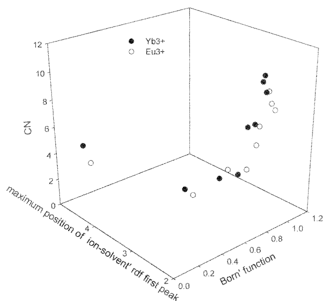
Figure 1. Plot of structural property vs. Born's function of bulk solvents at 298 K and 1 atm.
