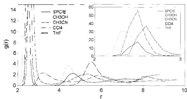
Figure 3. Radial distribution function of Yb 3+ ion in selected solvents.
