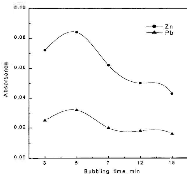
Figure 7. Bubbling time of a nitrogen gas for the effective sublation of the ion pairs.
