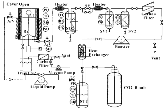
Fig. 1. Schematic diagram of carbon dioxide washer.
