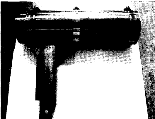
Fig. 4. Dry ice snow jet cleaning machine
