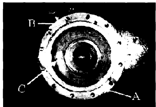
Fig. 5. Pump housing after dry ice snow cleaning
