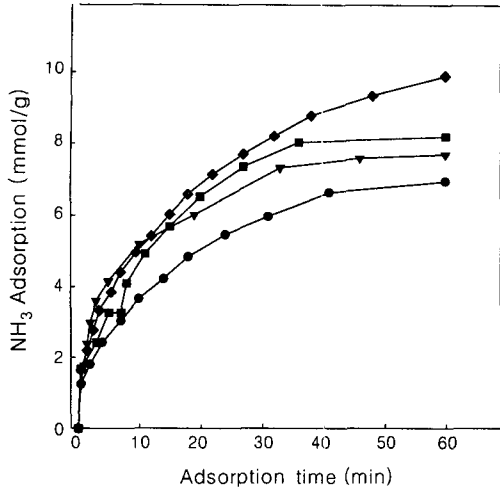
Figure 9. Comparison of the ammonia adsorption capacity of metal complexes of sulfonated PP-g-St (4.25 mmol H + /g) at 200 mmHg. Metal complex: (◆) Co 2+ , (■) Ni 2+ , (▼) Cu 2+ , (●) Zn 2+ .
