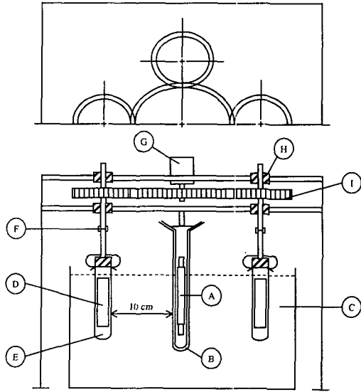
Figure 1. Schematic diagram of photoinduced graft polymerization apparatus. (A) UV lamp, (B) quartz immersion well, (C) water bath, (D) PP nonwoven, (E) pyrex tube containing the reaction mixture, (F) connecting device, (G) motor, (H) bearing house, and (I) conveyer belt.
