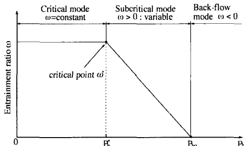
Fig. 3 Ejector operating mode
