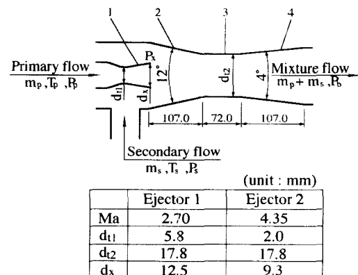
Fig. 1 Ejector configuration and dimensions
