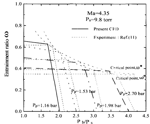
Fig.4 Entrainment ratio w vs P_p/P_s
