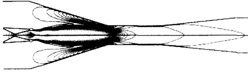
Fig. 2 Mach number contour for Ma=4.35 , d_1=2.0 , d_2=17.8 and d_x=9.3
