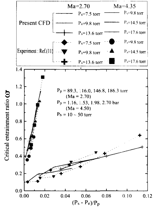
Fig. 8 Critical entrainment ratio w^* vs (P_s - P_e)/P_p
