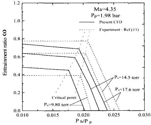
Fig. 5 Entrainment ratio w vs P_b/P_p
