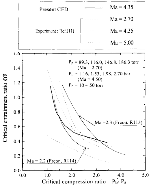
Fig. 9 Critical entrainment ratio w^* vs P_b^*/P_s
