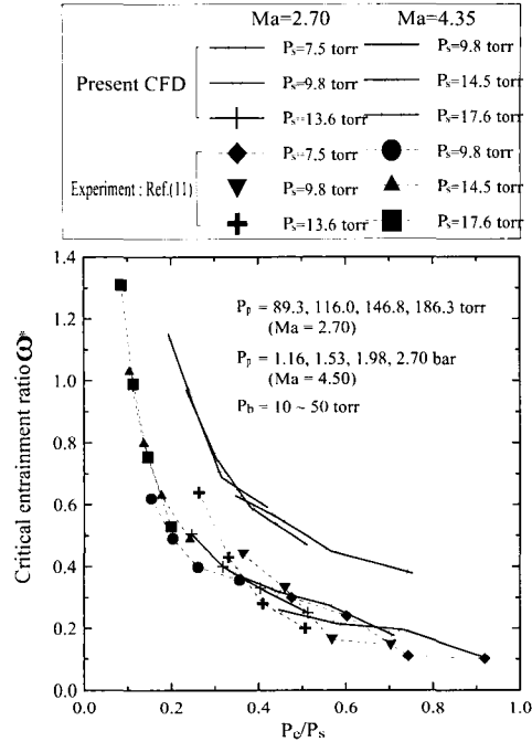
Fig. 6 Critical entrainment ratio w^* vs P_e/P_s
