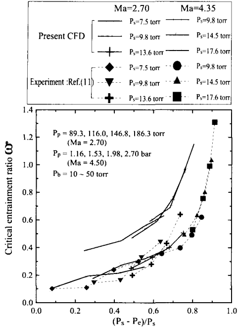
Fig. 7 Critical entrainment ratio w^* vs (P_s - P_e)/P_s
