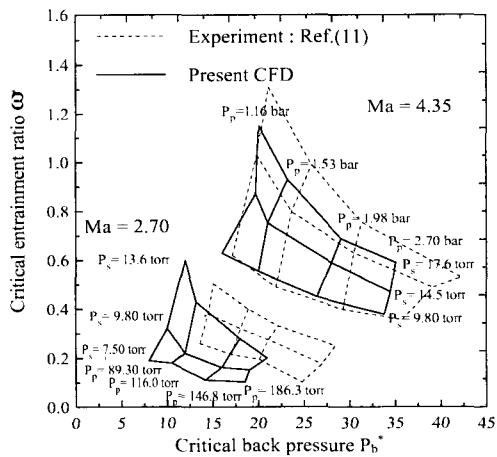
Fig. 10 Critical entrainment ratio w^* vs critical back pressure P_b^*/P_s
