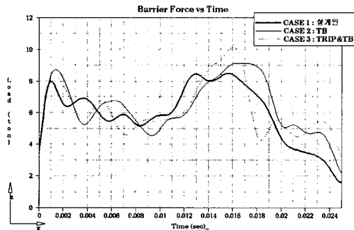
Fig. 1 Curve of load vs time
