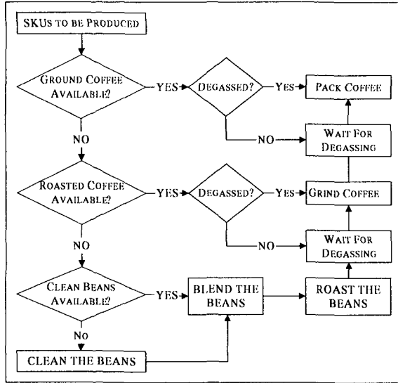
Figure 4: Scheduling Logic
