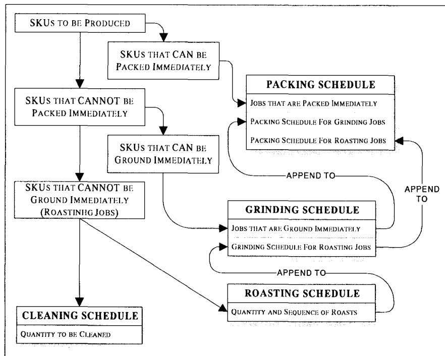
Figure 3: Scheduling Logic
