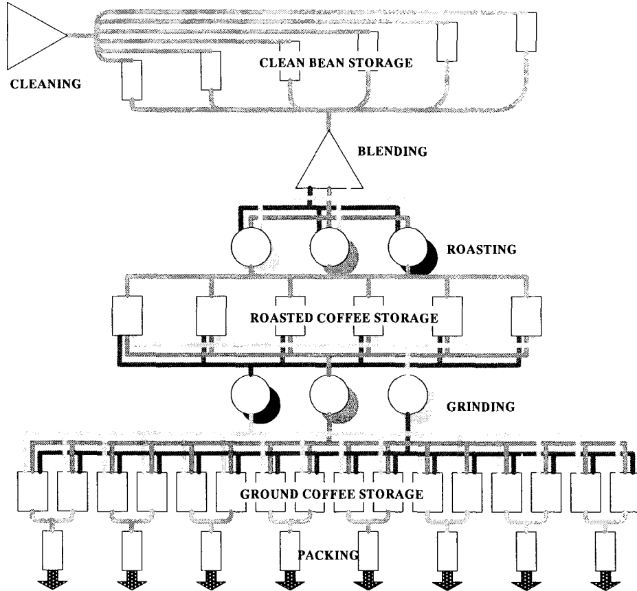
Figure 1: Schematic Representation of a Coffee Production Facility
