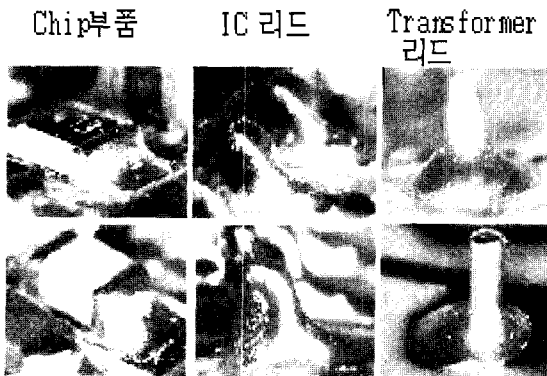
Fig. 5. Sn-Cu-Ni계 Solder Joint외관(초기)
