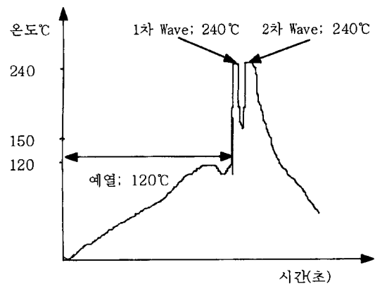
Fig. 3. Pb-Free Wave Soldering Profile(Set: 255°C, 실제 온도: 240°C).
