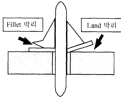
Fig. 6. Lift-off(fillet박리, Lan박리).
