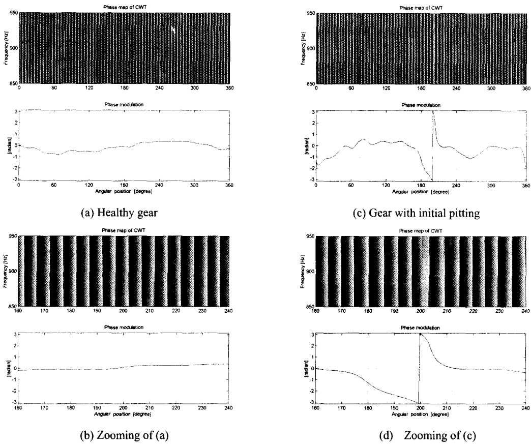
Fig. 6 Comparison the zoomed phase map of CWT with Phase modulation of McFadden
