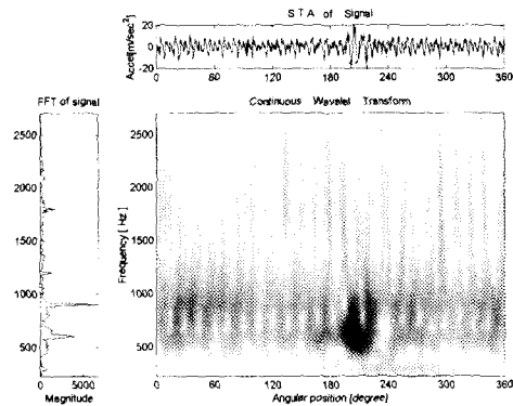
(b) Gear with tip breakage
