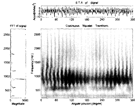
(a) Healthy Gear
