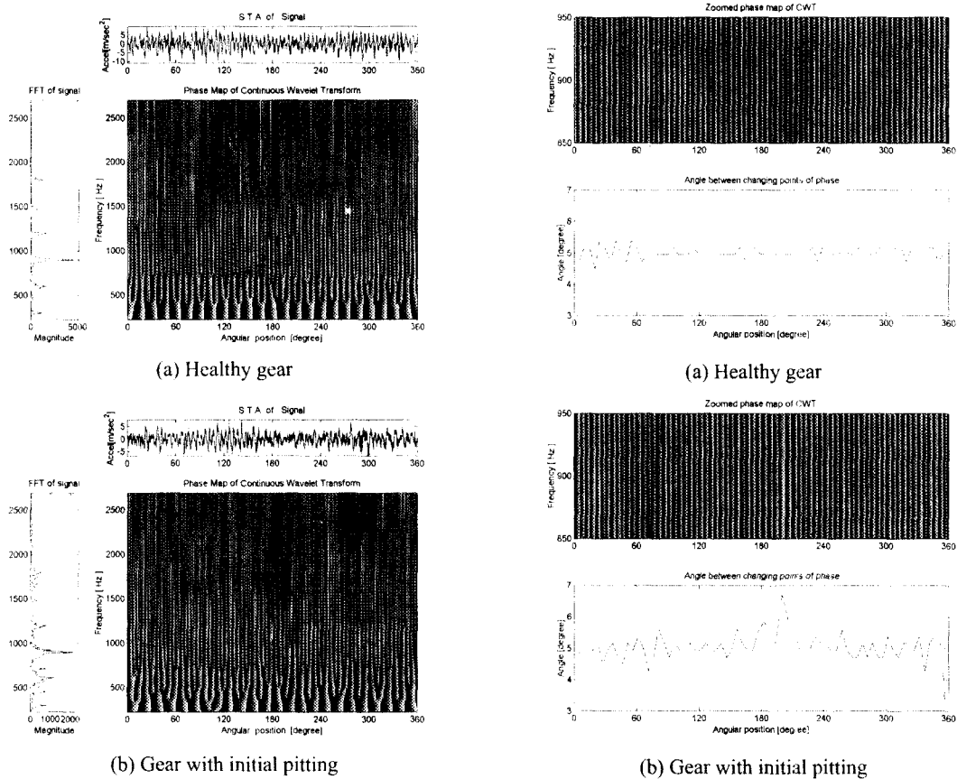
Fig. 4 Phase map of CWT
