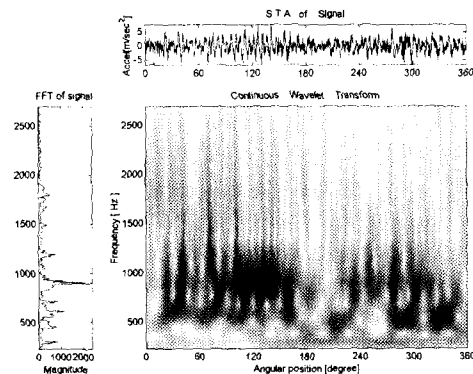
(c) Gear with initial pitting
