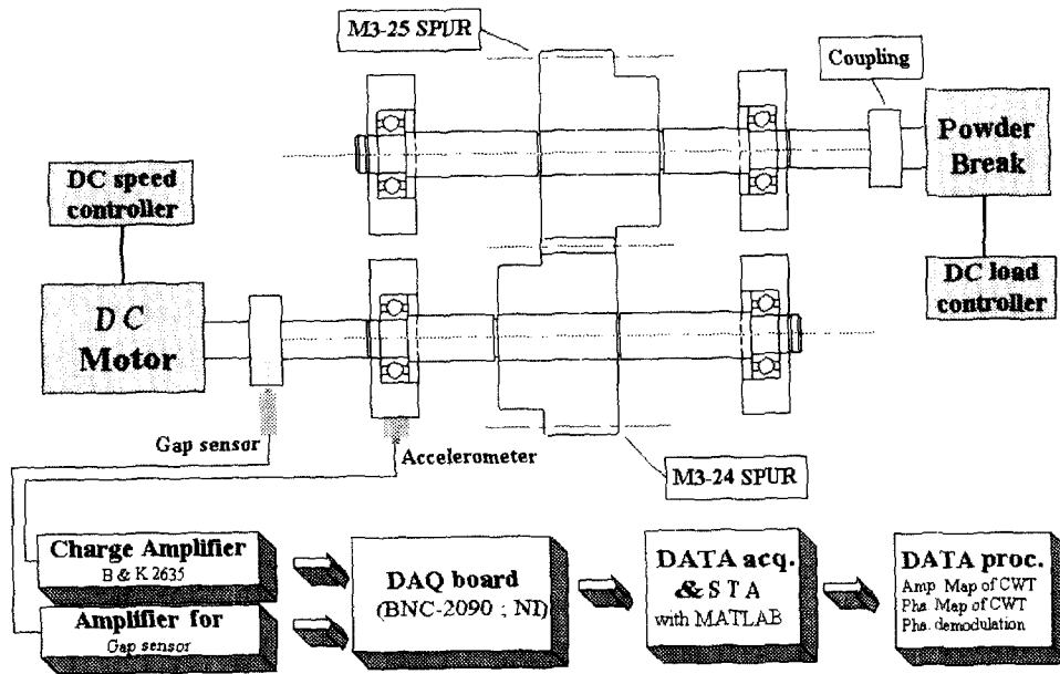
Fig. 1 Schematic diagram of Test Rig for gear fault detection
