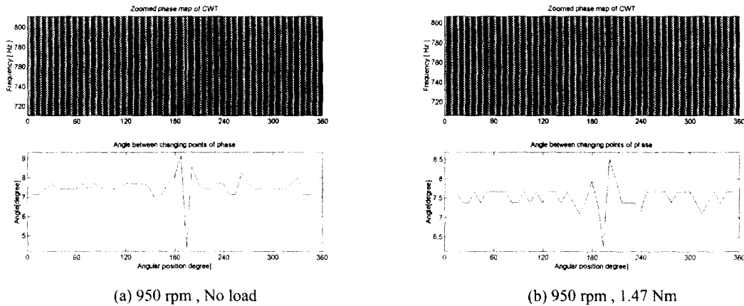
Fig. 7 Zoomed phase map of CWT in other experimental conditions
