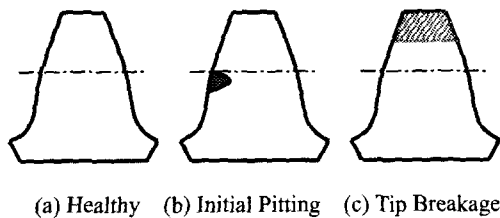
Fig. 2 Details of gear fault for experiment
