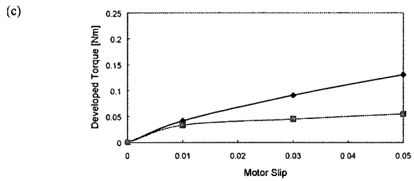
Fig. 13 Comparison of the developed torque between the silicon steel rotor system and the composite rotor system w.r.t. motor slip.
