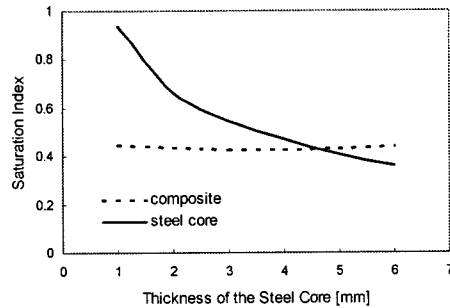
Fig. 6 Magnetic saturation index ( B/B_{saturated} ) w.r.t. the core thickness.
