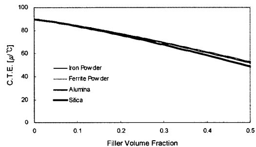
Fig. 17 Calculation results of coefficient of thermal expansion w.r.t. powder volume fraction for various powders using Wang's formula.
