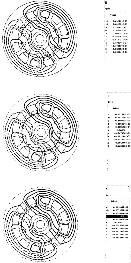
Fig. 10 Flux distribution of composite rotor w.r.t. the position of conductor bars.
