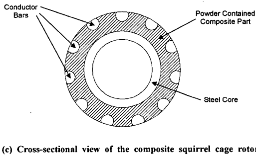
Fig. 1 Configurations of composite squirrel cage rotor.
