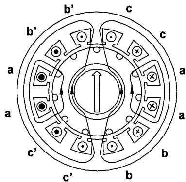
Fig. 2 Schematic diagram of magnetic flux of a 2 pole 3 phase motor.
