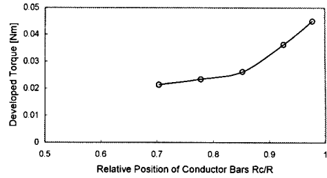
Fig. 8 Developed torque of the composite rotor w.r.t. the radial position of conductor bars.
