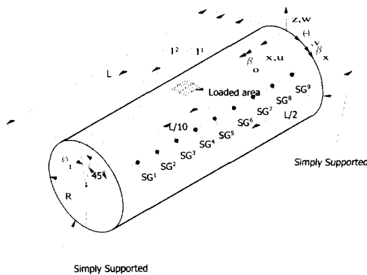
Fig. 1 Analysis model of composite cylindrical shell
