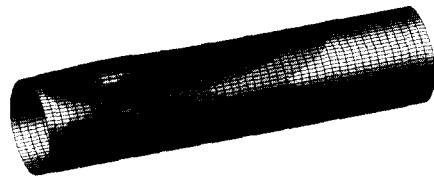
Fig. 3 Impact response shape at L/5 location under 4,450 N(1,000 lbs) loading
