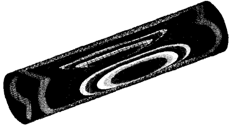
Fig. 2 1st modeshape of the composite shell
