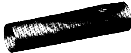
Fig. 5 Impact response shape at 4L/5 location under 4,450 N(1,000 lbs) loading
