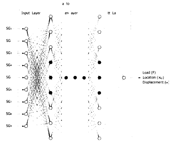
Fig. 10 Model of neural networks for identification of loads characteristics by the side strain
