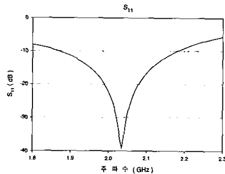
(a) S_{11}
