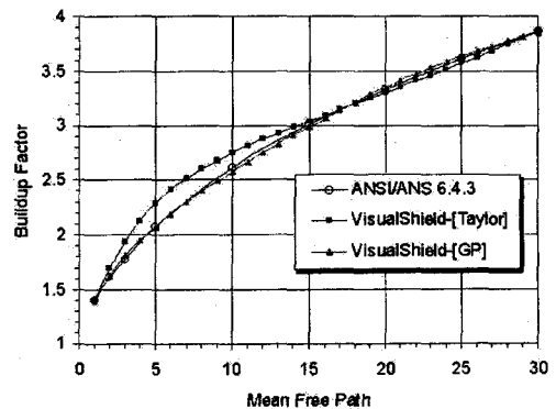
(a) Shield thickness
