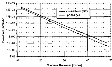
Fig. 8. Results of shielding analysis of the purification filter using VisualShield and ISOSHLD.
