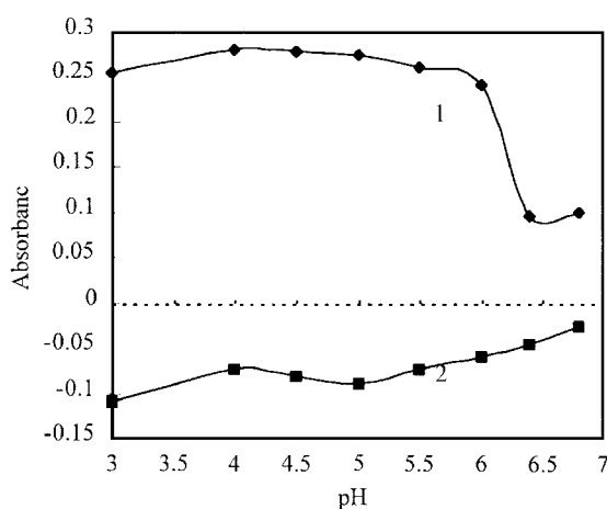
Figure 4. Effect of pH on absorption of Ge ( 10 \mu\text{g} )- o -CPF complex solution: 1- \Delta 4 at 530 nm and 2- \Delta 4' at 460 nm.
