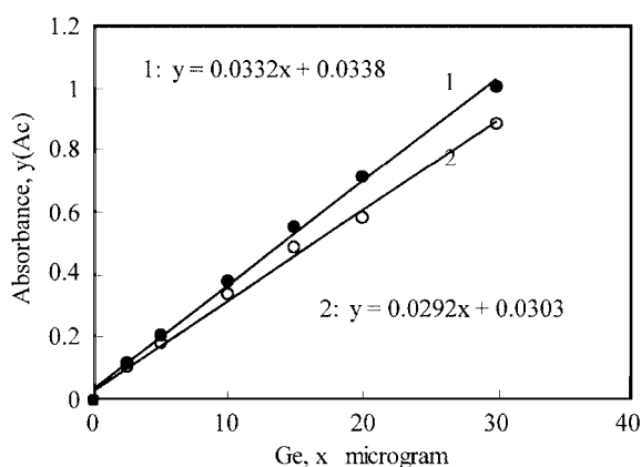
Figure 8. Calibration curves for the determination of germanium at 530 nm: 1-Δc, 2-ΔΔ.
