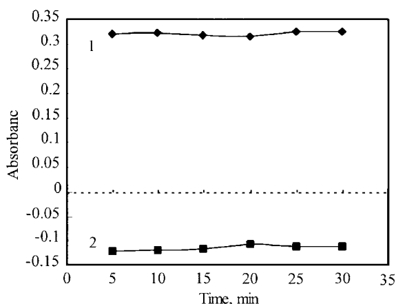
Figure 7. Effect of the reaction time on absorption of Ge (10 µg)- o -CPF complex solution: 1-ΔΔ at 530 nm and 2-ΔΔ at 460 nm.
