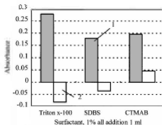
Figure 5. Effect of the different surfactant on absorption of Ge ( 10 \mu\text{g} )- o -CPF complex solution: 1- \Delta 4 at 530 nm and 2- \Delta 4' at 460 nm.
