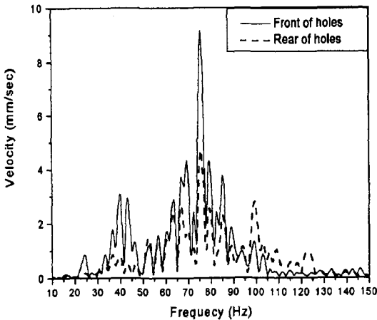
Fig. 11. Fourier transform of transverse component velocities
