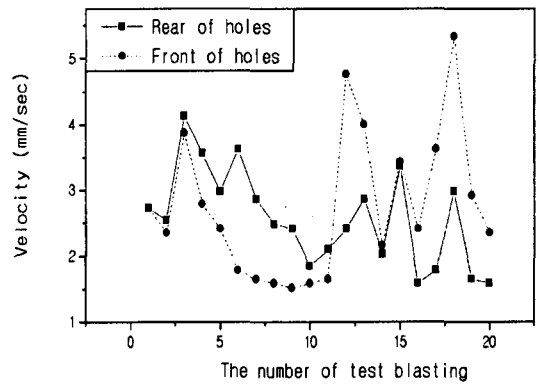
Fig. 9. Comparison of longitudinal component velocities
