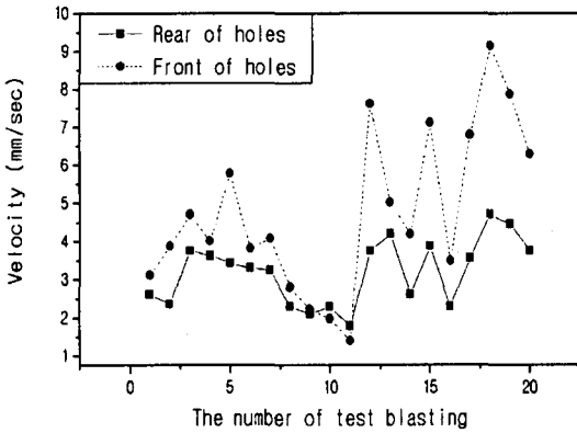
Fig. 7. Comparison of transverse component velocities
