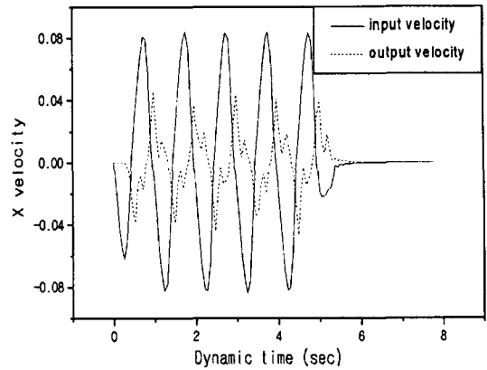
Fig. 2. Input velocity wave and output velocity wave
