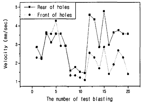
Fig. 10. Comparison of PVS component velocities
