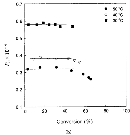
Figure 4. ( P_n )s of PVAc (a) and PVA (b) obtained at three different polymerization temperatures with conversions (ADMVN concentration of 1 \times 10^{-4} mol/mol of VAc and solvent concentration of 0.25 mol/mol of VAc).
