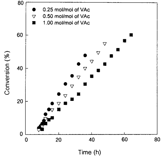
Figure 2. Conversion of VAc into PVAc at 30 °C using ADMVN concentration of 1 \times 10^{-4} mol/mol of VAc with polymerization time.
