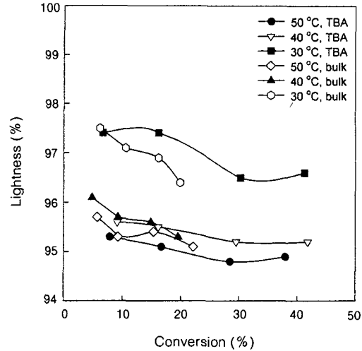
Figure 9. Effects of conversion and polymerization temperature on the lightness of PVA derived from PVAc obtained by solution polymerization in TBA and by bulk polymerization, respectively.
