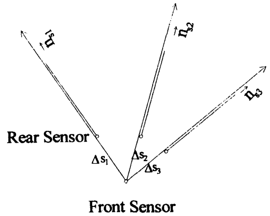
Fig. 2. Schematic of Four Sensor Probe
