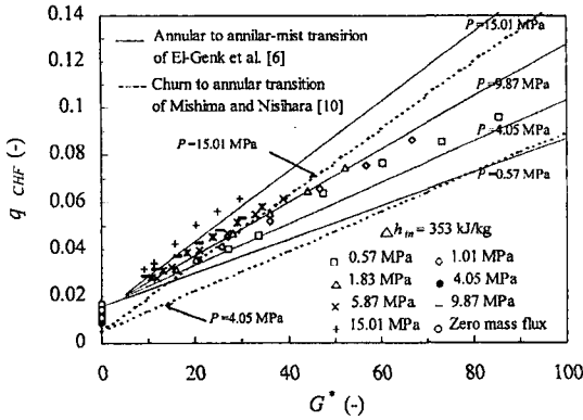
Fig. 6. Dimensionless CHF as a Function of Dimensionless Mass Flux
