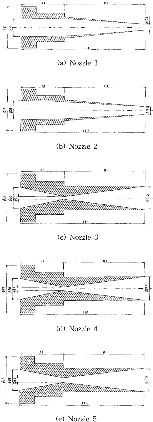
Fig.3 Primary nozzle configurations(unit:mm)
