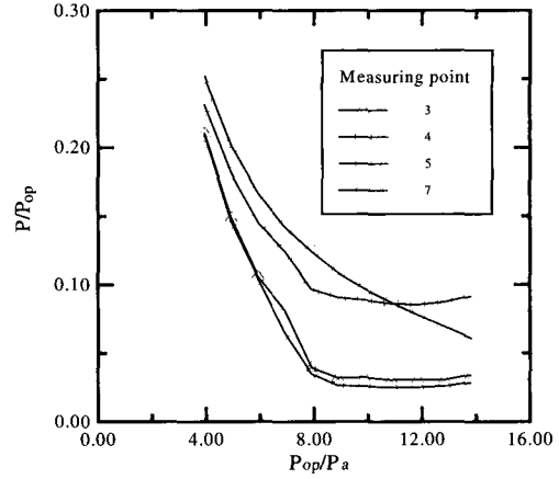
Fig.5 Pressure variation in supersonic ejector system (Ejector throat area ratio : 7.49)
