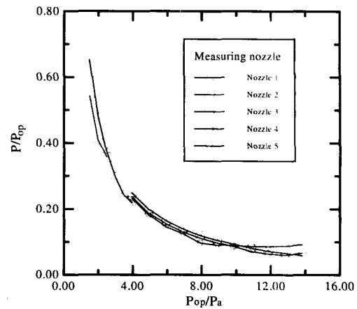
Fig.7 Pressure in mixing tube
