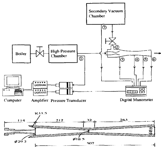
Fig.1 Experimental facility
