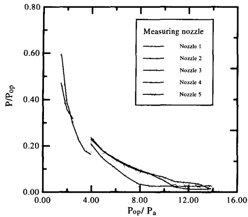
Fig.6 Secondary chamber pressure
