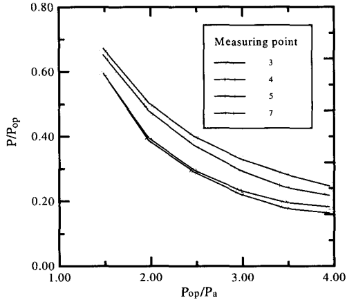
Fig.4 Pressure variation in subsonic ejector system (Ejector throat area ratio : 4.0)
