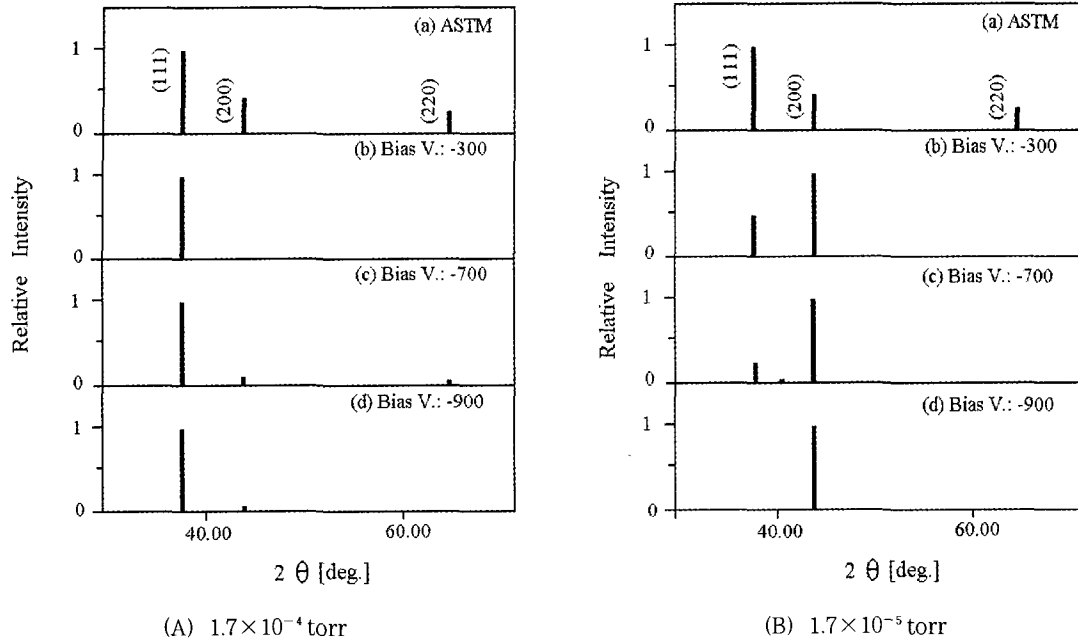
Fig. 4. X-ray diffraction patterns of Ag films deposited at various deposition conditions.
