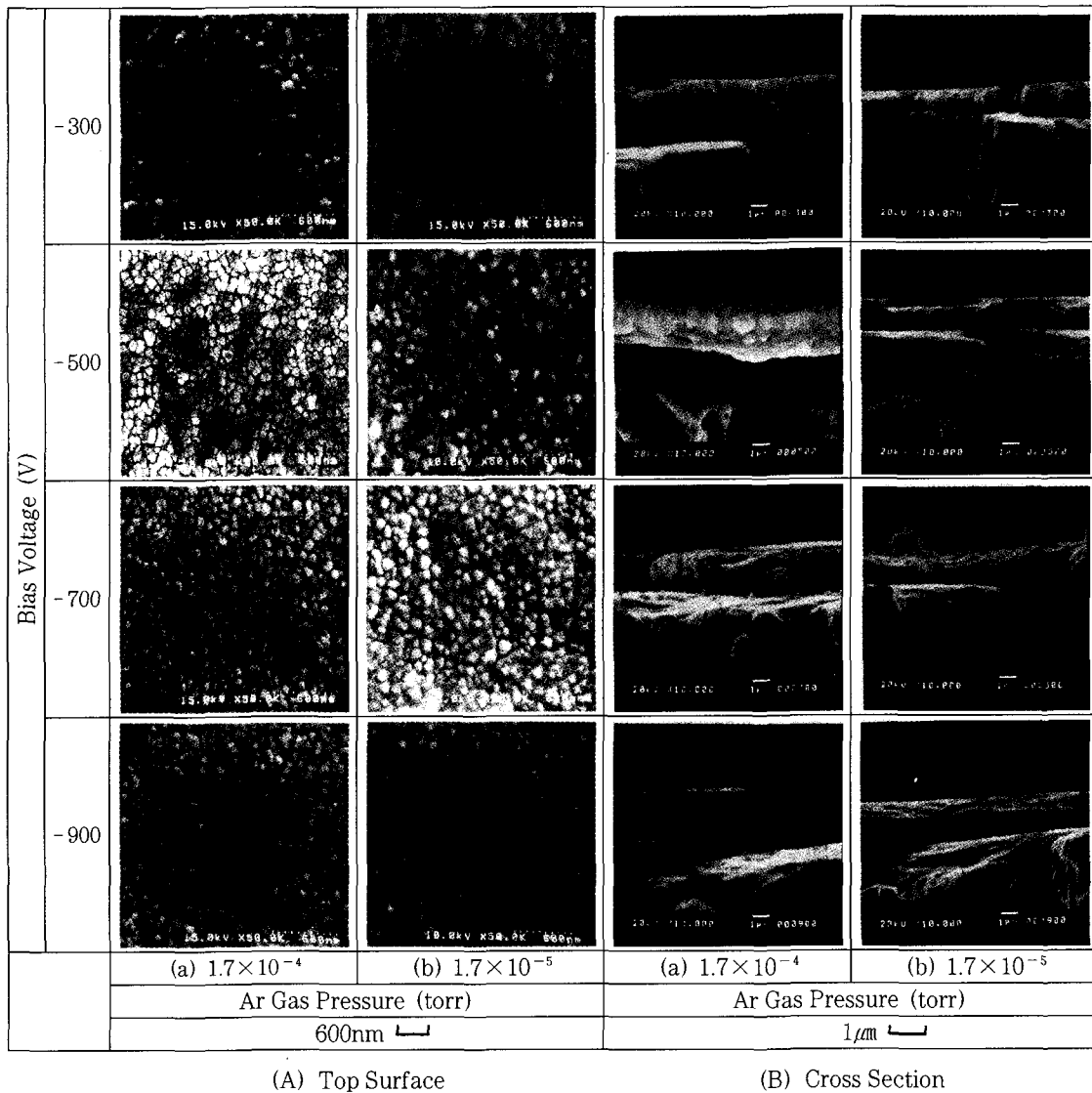
Fig. 3. SEM photographs of top surface and cross section for Ag films on the substrate of STS 440C.
