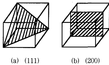
Fig. 5. Lattice plane of cubic.
