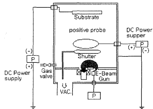
Fig. 1. Schematic diagram of ion plating apparatus.
