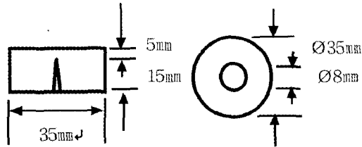
Fig. 2. View of schematic diagram for specimen.
