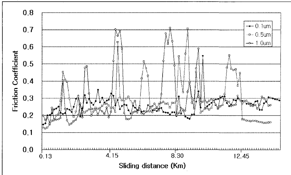
Fig. 8. Variation of friction coefficient with sliding distance on the thickness of Ag films deposited at 1.7 \times 10^{-4} torr. (Bias V.: -300V)
