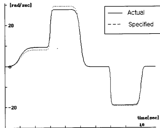
Fig. 7. Tracking performance for a sigmoid reference.
