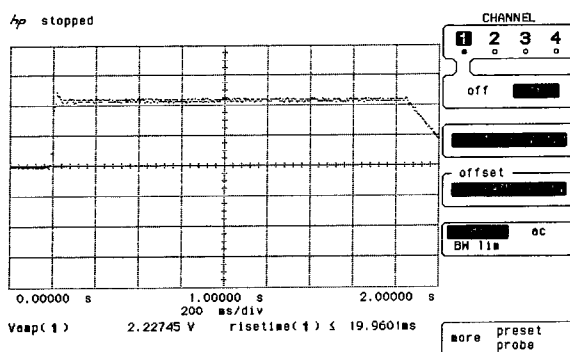
Fig. 10. Tracking performance of control algorithm to DC servo motor.
