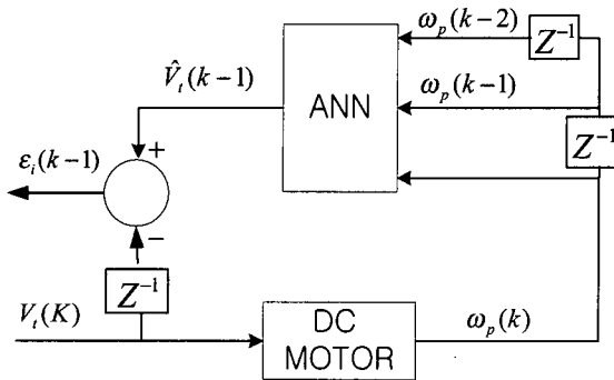
Fig. 3. Structure of the ANN identifier.
