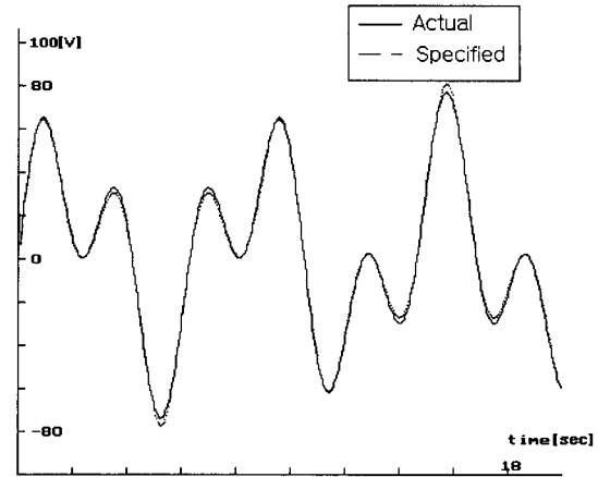
Fig. 4. Actual and estimated terminal voltages of the DC servo motor.
