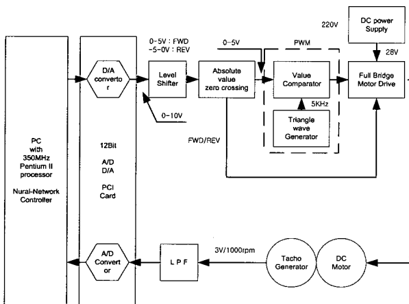
Fig. 9. Overall structure of experimented control system.
