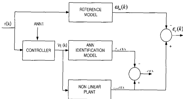
Fig. 2. ANN Based identification and control system.
