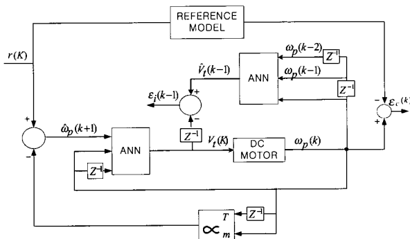
Fig. 5. Overall structure of the controller.
