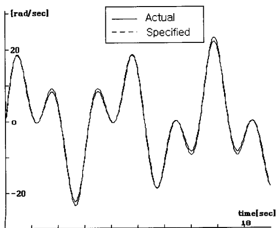
Fig. 6. Tracking performance for a sinusoidal reference trajectory.
