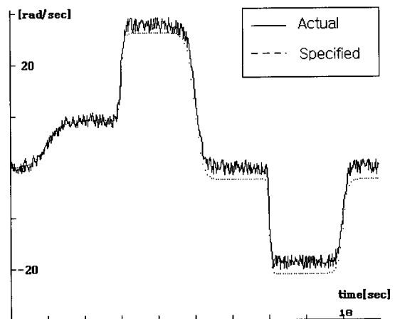
Fig. 8. Tracking performance for a sigmoid reference track with measurement noise.
