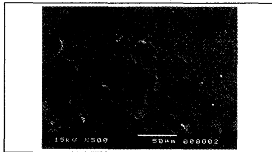
Fig. 11. SEM micrographs of the worn surface of PTFE20%-PI80%
