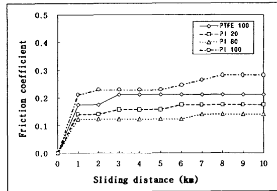
Fig. 4. Relationship between friction coefficient and sliding distance according to the rate of filling of polyimide for sliding speed at 1.88m/s
