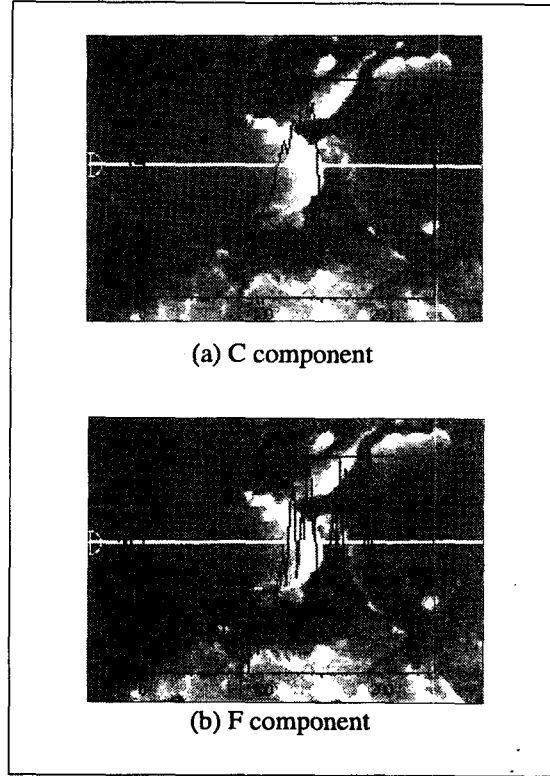
Fig. 14. EDS micrographs of the worn surface of PTFE20%-PI80%
