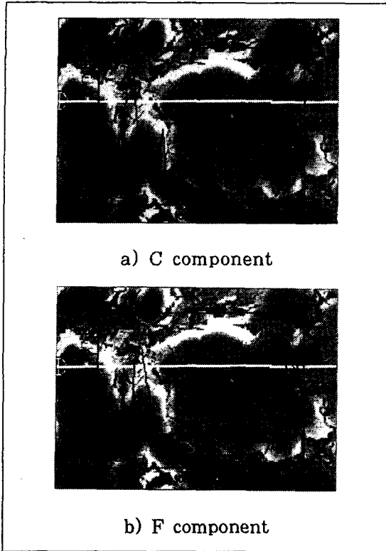
Fig. 13. EDS micrographs of the worn surface of PTFE80%-PI20%
