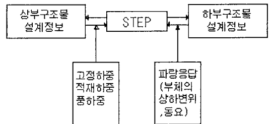
Fig. 3 Information exchange between super-structure and floating structure
