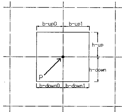
Fig. 5 Attribute for tributary area
