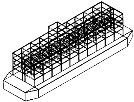
Fig. 9 Structural modeling of floating hotel
