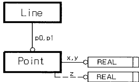
Fig. 4 Express-G
