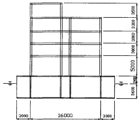
Fig. 8 Cross section
