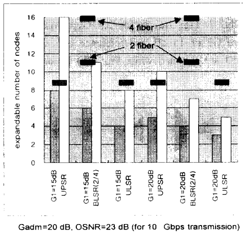
(b) G2=20 dB, OSNR=23 dB assumed for 10 Gbps transmission
