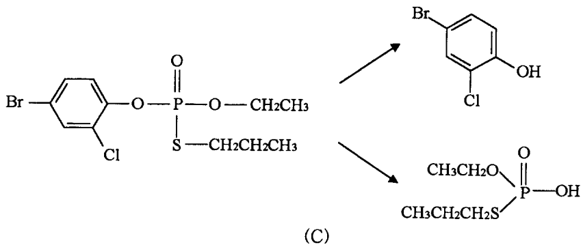
Fig. 12. Mass spectra of (peak1) and (peak2) of degradation products of profenofos and their proposed chemical structure(C).
