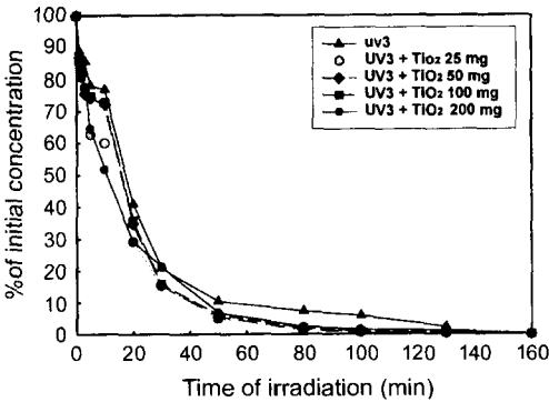
Fig. 7. Photolysis of profenofos in the UV 3(24W) system with TiO 2 powder amount.
