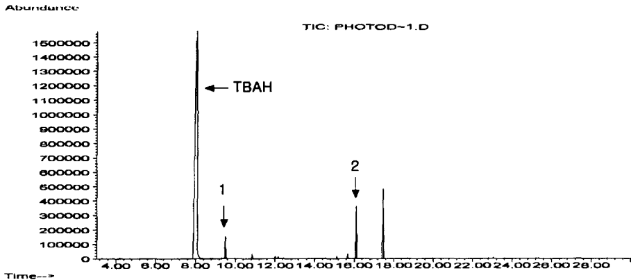
Fig. 11. Total ion chromatograms of degradation products of profenofos by photolysis.
