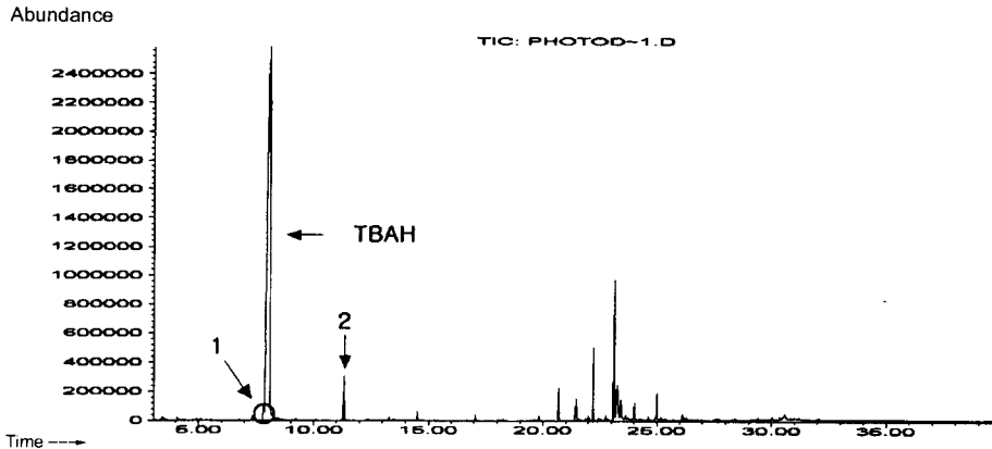
Fig. 9. Total ion chromatograms of degradation products of phosphamidon by photolysis.
