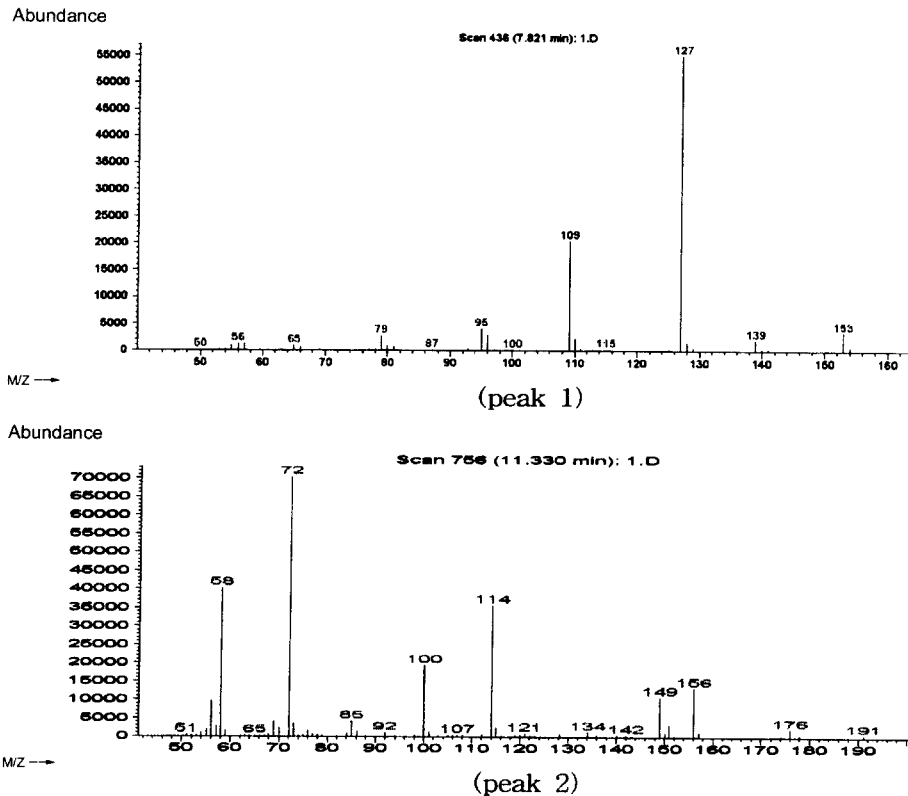
Fig. 10. Mass spectra of (peak 1) and (peak 2) of degradation products of phosphamidon and their proposed chemical structure(C).
