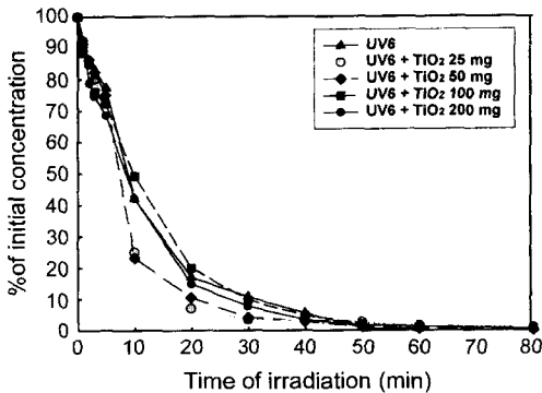
Fig. 8. Photolysis of profenofos in the UV 6(48W) system with TiO 2 powder amount.
