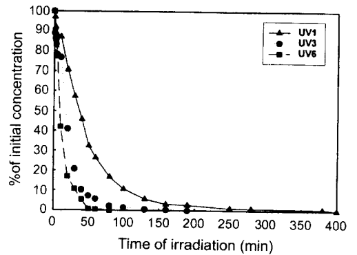
Fig. 5. Photolysis of profenofos in the UV system with the illumination of UV 1(8W), UV 3(24W) and UV 6(48W).
