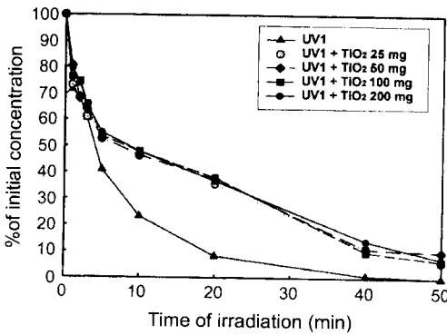
Fig. 2. Photolysis of phosphamidon in the UV 1(8W) system with TiO 2 powder amount.
