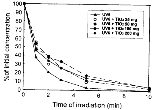
Fig. 4. Photolysis of phosphamidon in the UV 6(48W) system with TiO 2 powder amount.
