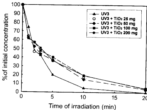
Fig. 3. Photolysis of phosphamidon in the UV 3(24W) system with TiO 2 powder amount.
