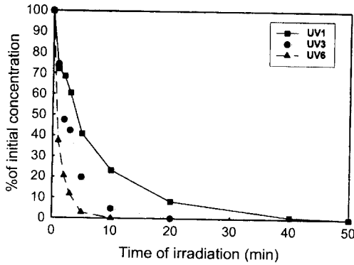
Fig. 1. Photolysis of phosphamidon in the UV system with the illumination of UV 1(8W), UV 3(24W) and UV 6 (48W).
