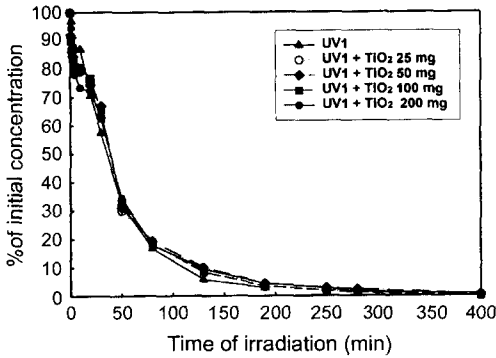
Fig. 6. Photolysis of profenofos in the UV 1(8W) system with TiO 2 powder amount.
