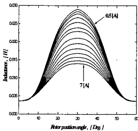
(b) Inductance profiles
