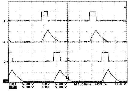
(a) Gate signal and corresponding phase current
