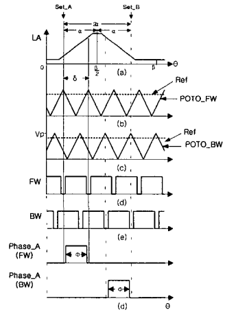
Fig. 3 Switching patterns of the phase switch
