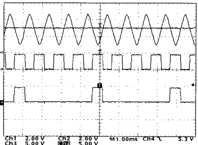
(b) Output signals of photo Tr., encoder and gate signal
