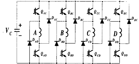
(c) Classic inverter circuit for SRM drive
