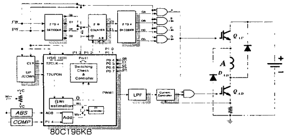
Fig. 5 Block diagram of the controller
