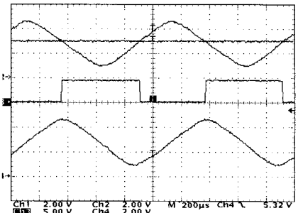
(a) Output signals of photo Tr. and encoder
