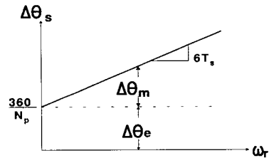
Fig. 1 Error of switching angle to speed
