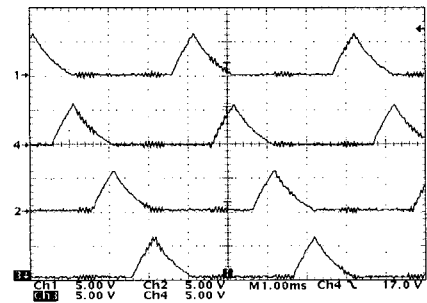
(b) Each phase currents
