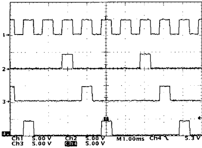
(c) Gate signal and corresponding encoder signal
