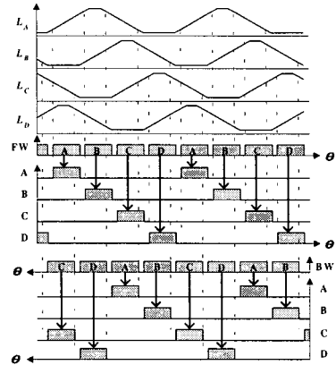
Fig. 4 Gate signal of each phase when SRM is rotating in the forward and backward directions by the proposed encoder
