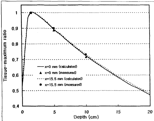
Fig. 3. The measured (symbols) and calculated (lines) tissue maximum ratios as a function of the independent jaw positions from the central axis for 50 mm diameter collimator cone. The measurements were done with one independent jaw positions at 15.5 mm and 0 mm from the central axis, respectively, using 0.009 cc micro ion chamber (Extradin A-14). All the measured data were within 0.3% error range of the calculated values.
