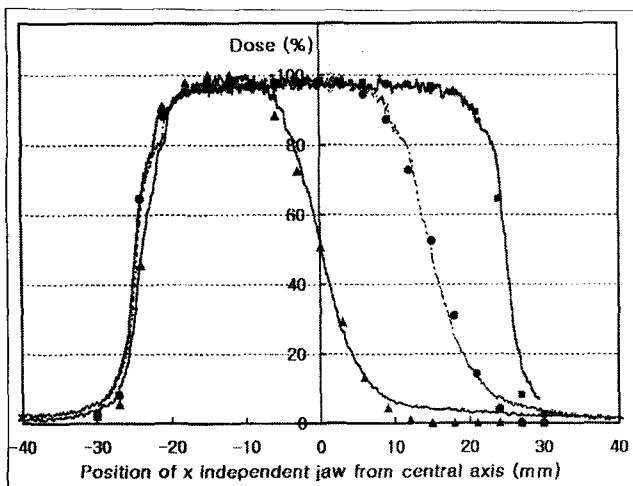
Fig. 4. The measured (lines) and calculated (symbols) dose profiles at 5 cm depth for 50 mm diameter collimator cone. The measurements were performed with one independent jaw positions at 30 mm (unblocked), 15.5 mm, and 0 mm from the central axis, respectively, using film dosimetry procedure (Kodak XV-2 film and VIDAR VXR-12 scanner).
