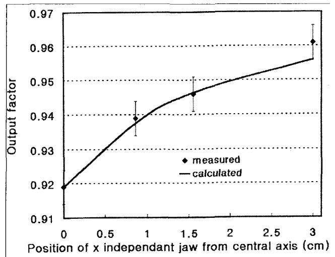
Fig. 2. The measured (symbol) and calculated (line) output factors as a function of the independent jaw positions from the central axis for 50 mm diameter collimator cone. The measurements were done with one independent jaw positions at 30 mm (unblocked), 15.5 mm, 8.6 mm, and 0 mm from the central axis, respectively, using 0.009 cc micro ion chamber (Exradin A-14). All the measured data were within 0.5% error range of the calculated values (error bar).
