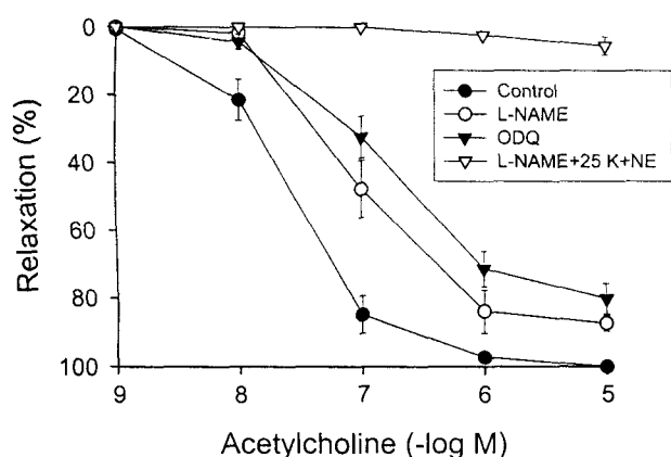
Fig. 1. Average concentration-response curves for the relaxant effects of ACh in the absence (●) and presence of 0.1 \text{ mM} L-NAME (○) or in the presence of ODQ (▼) or in the presence of 1 \mu\text{M} NE, L-NAME plus 25 \text{ mM} KCl (▽). Responses are expressed as the percentage of contraction elicited by NE ( 1 \mu\text{M} ) before the addition of ACh. Each point represents mean of 6–10 rings and S.E.M. is shown by vertical bar. L-NAME, \text{N}^G -nitro-L-arginine methyl ester hydrochloride.
