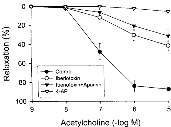
Fig. 3. Effects of \text{K}^+ channel blockers on ACh-induced relaxation in endothelium-intact L-NAME (0.1 mM)-pretreated segments of the rabbit renal artery precontracted with NE (1 \mu\text{M} ). ●, Control; ○, in the presence of iberiotoxin (0.3 \mu\text{M} ); ▼, in the presence of iberiotoxin (0.3 \mu\text{M} ) plus apamin (1 \mu\text{M} ); ▽, in the presence of 4-AP (5 mM). Responses are expressed as the percentage of contraction elicited by NE before the addition of ACh. Each point represents mean of 5–8 rings and S.E.M. is shown by vertical bar. L-NAME, \text{N}^G -nitro-L-arginine methyl ester hydrochloride.
