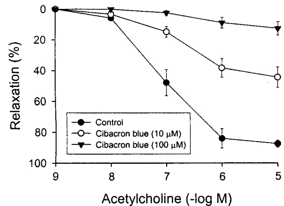
Fig. 4. Effects of \text{P}_{2Y} purinoceptor antagonist, cibacron blue on ACh-induced relaxation in endothelium-intact L-NAME (0.1 mM)-pretreated segments of the rabbit renal artery precontracted with NE (1 \mu\text{M} ). ●, Control; ○, in the presence of 10 \mu\text{M} cibacron blue; ▼, in the presence of 100 \mu\text{M} cibacron blue. Responses are expressed as the percentage of contraction elicited by NE before the addition of ACh. Each point represents mean of 6 rings and S.E.M. is shown by vertical bar. L-NAME, \text{N}^G -nitro-L-arginine methyl ester hydrochloride.
