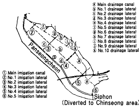
<Fig. 2> Irrigation and drainage canal network
