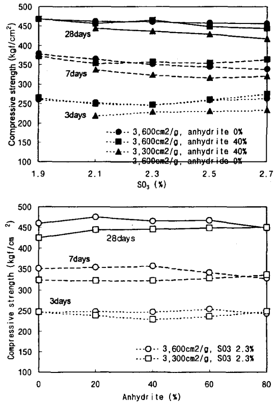
Fig.8 Compressive strength of cement mortars with same W/C at 20°C
