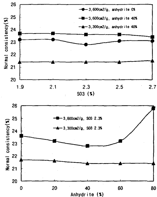
Fig. 1 Normal Consistency of cement pastes
