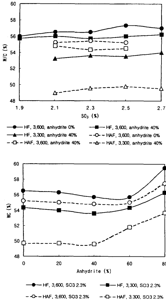
Fig.7 W/C of cement mortars with same flow value at 35°C
