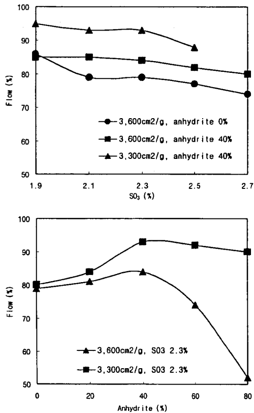
Fig.5 Mortar flows of cements with same W/C at 20°C
