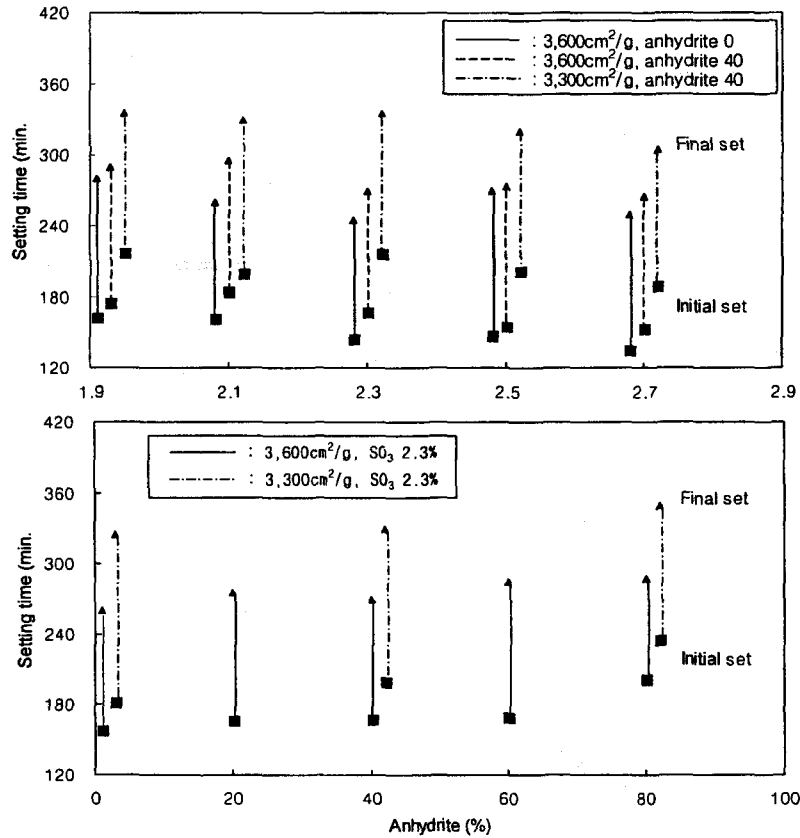
Fig. 2 Setting time of cement pastes
