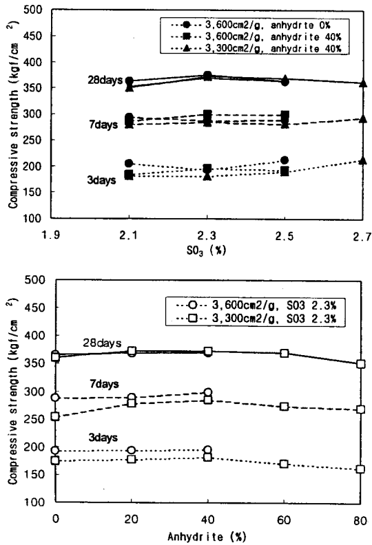
Fig. 9 Compressive strength of cement mortars with same flow and admixture at 35°C
