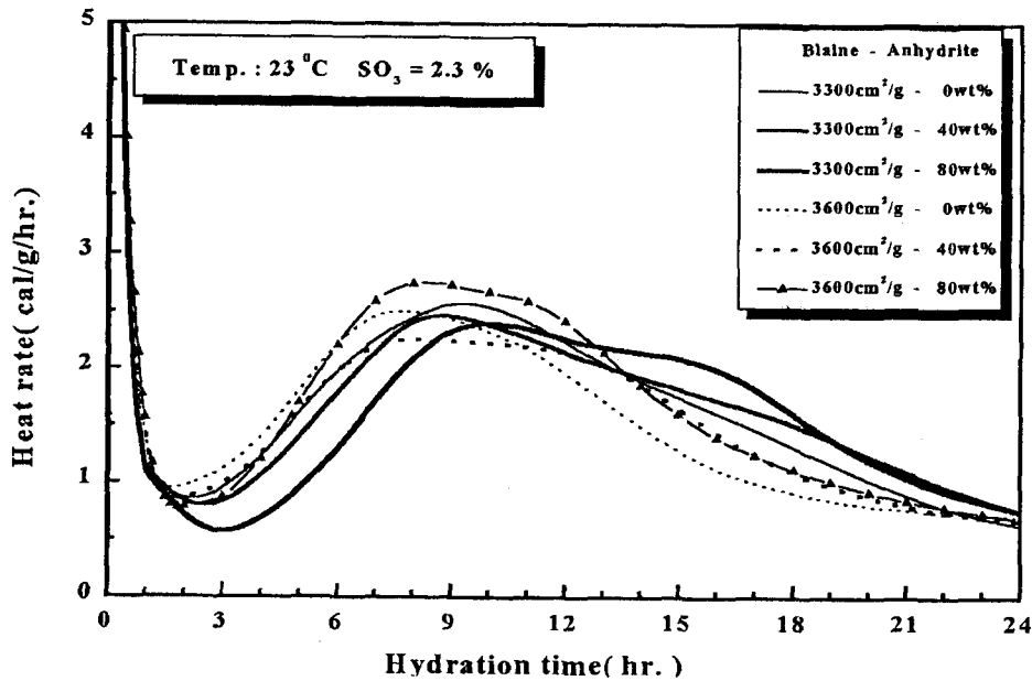
Fig.3 Heat evolution rate curves of cements at 23°C
