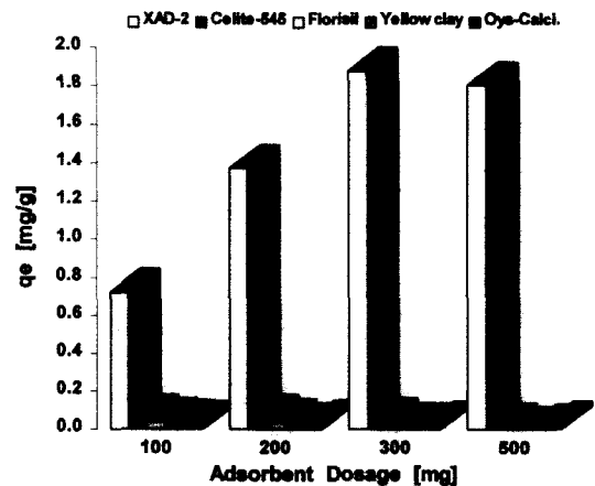
Fig. 2. Geosmin adsorption capacity of Adsorbent.
