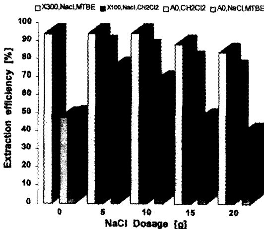
Fig. 4. The effect of extraction efficiency on NaCl dosage.
