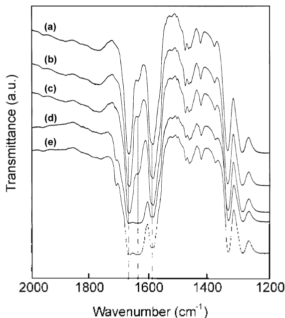
Figure 1. FT-IR spectra of 2-EAQ-Y after (a) evacuation at 200 °C for 2 h. (b) adsorption of 10 torr of H 2 at RT for 20 min. (c) adsorption of 10 torr of O 2 at RT for 20 min.. (d) heating at 60 °C for 10 min.. and (e) evacuation at room temperature.
