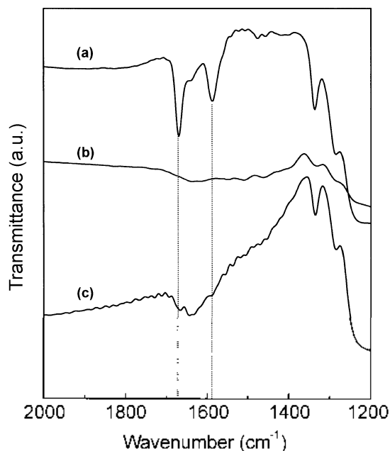
Figure 2. FT-IR spectra of 2-EAQ/Pd-Y after (a) evacuation at 200 °C for 2 h. (b) adsorption of 10 torr of H 2 at RT for 20 min.. and (c) adsorption of 10 torr of O 2 at RT for 20 min.
