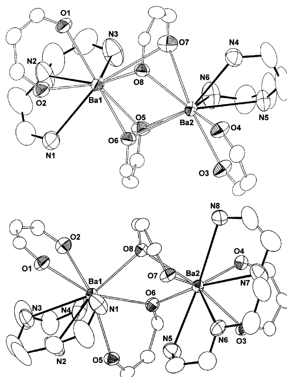
Figure 1. Structure and labeling of (a) [\text{Ba}(\text{THD})_2(\text{diethylenetriamine})]_2 (I) and (b) [\text{Ba}(\text{THD})_2(\text{triethylenetetramine})]_2 (II). Thermal ellipsoids as drawn by ORTEP represent the 30% probability surfaces. Hydrogen atoms and 'Bu carbon atoms in THD ligand have been omitted for clarity.
