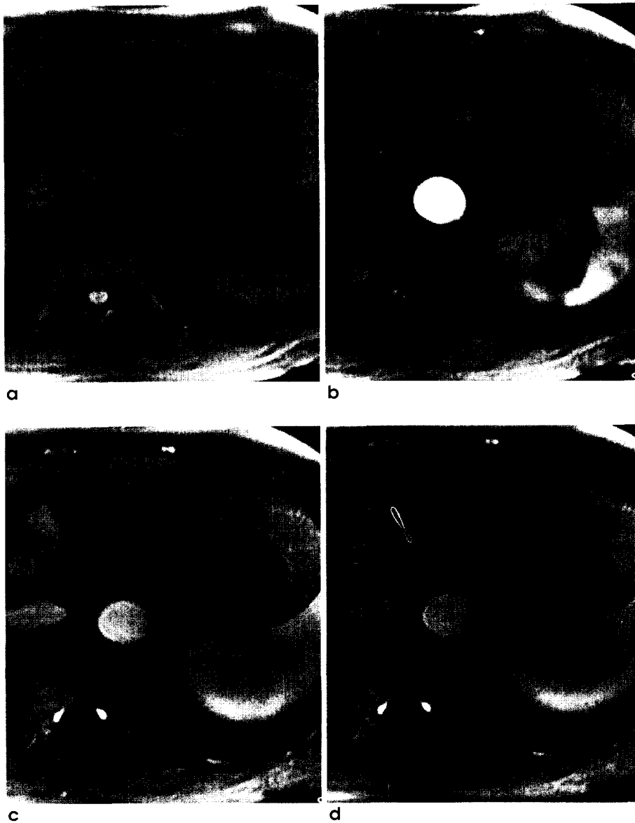
Fig. 2. Small hepatocellular carcinoma with iso-signal intensity on unenhanced T1-weighted images delineated solely by a single phase of contrast enhancement. (a) Unenhanced T1-weighted gradient echo image shows no definite evidence of focal lesion in left lobe of the liver. (b) First phase contrast-enhanced image obtained 10 sec after start of contrast injection shows nodular contrast enhancement (arrow). Second (c) and third (d) phase FLASH MR images obtained 35 and 60 sec after start of contrast injection show lack of enhancement.
