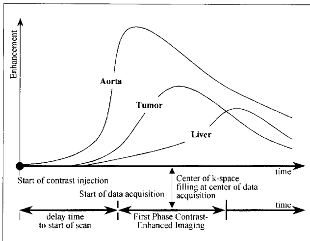
Fig. 1. Optimal imaging of arterial-dominant phase during dynamic MR imaging of the liver can be accomplished by proper timing of data acquisition depending on the relative difference of contrast-enhancement in aorta, tumor and liver parenchyma.
