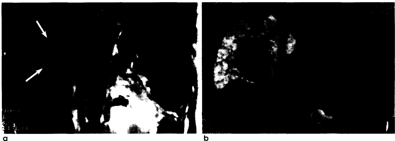
Fig. 5. Improved lesion-to-liver contrast of hepatic lymphoma with mangafodipir (Mn-DPDP). Precontrast T1-weighted gradient echo image (a) shows solitary lesion (arrows). Postcontrast image shows marked hepatic enhancement (b). (From Dr. K.C. Cho at New Jersey Medical School).
