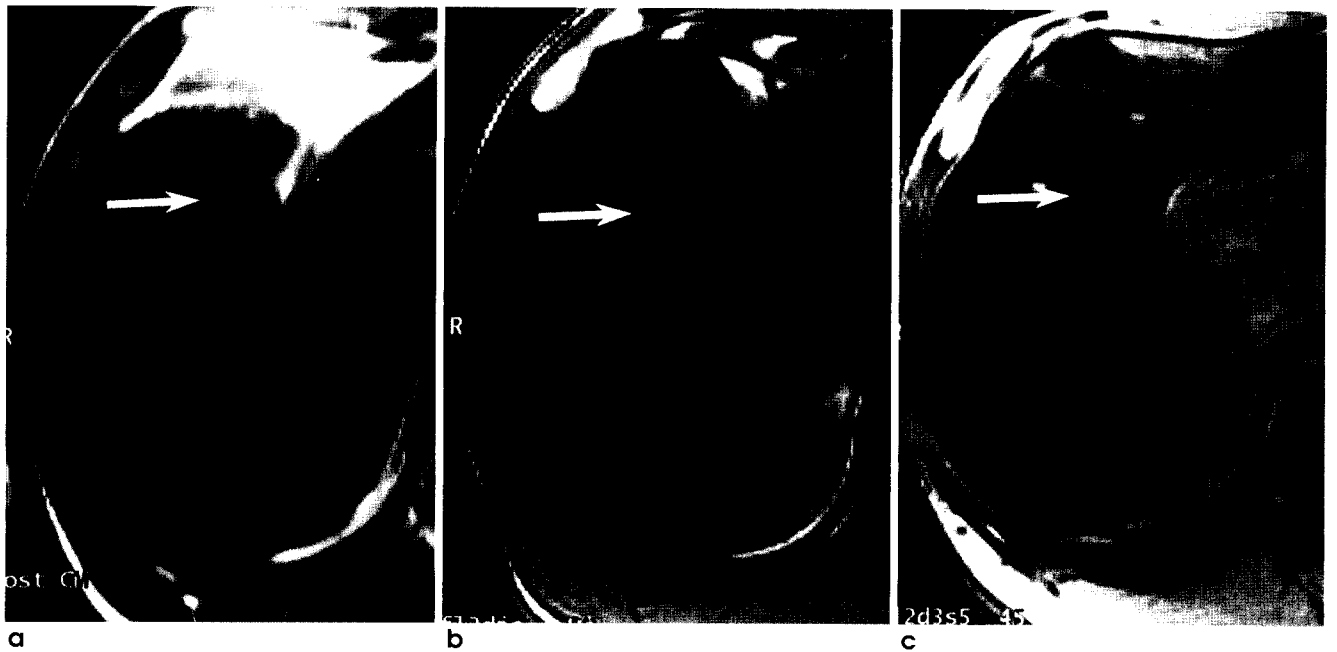
Fig. 3. Enhanced detection of small hepatocellular carcinoma using superparamagnetic iron oxide on T2*-weighted imaging. Postcontrast T2-weighted turbo spin echo (TR/TE = 1859msec/80msec, echo train length = 5) image (a) and T1-weighted gradient echo (TR/TE/flip angle = 140msec/2.7msec/90°) image (b) show slightly high signal intensity nodule in right lobe of the liver (arrows). Gradient echo image with longer echo time (7.7msec) for T2* effect with 45° flip angle (c) shows improved delineation of the lesion with good image resolution.
