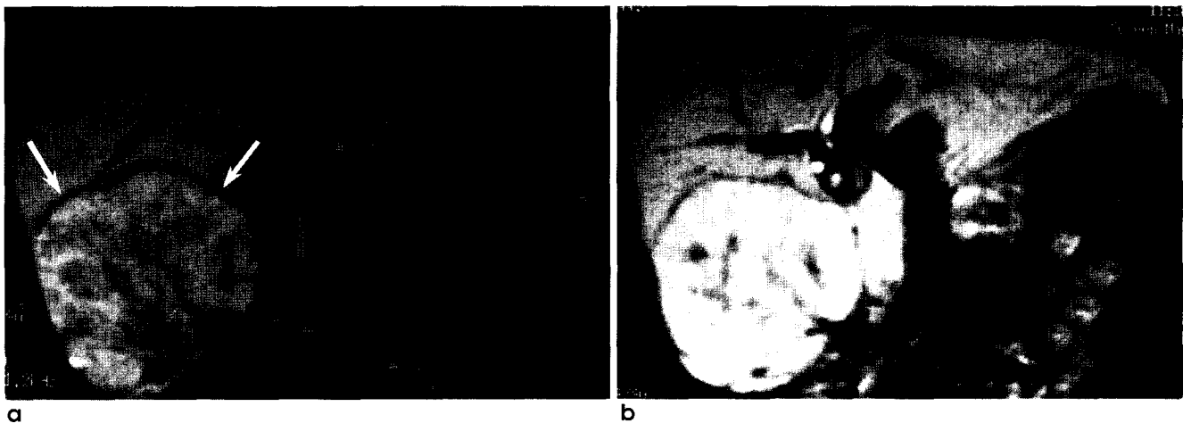
Fig. 6. Contrast enhancement of well-differentiated hepatocellular carcinoma with mangafodipir (Mn-DPDP). Precontrast T1-weighted gradient echo (a) shows a huge mass with high signal intensity in right lobe of the liver (arrows). Postcontrast image (b) shows marked enhancement of tumor as well as hepatic parenchyma. (From Dr. K.C. Cho at New Jersey Medical School).
