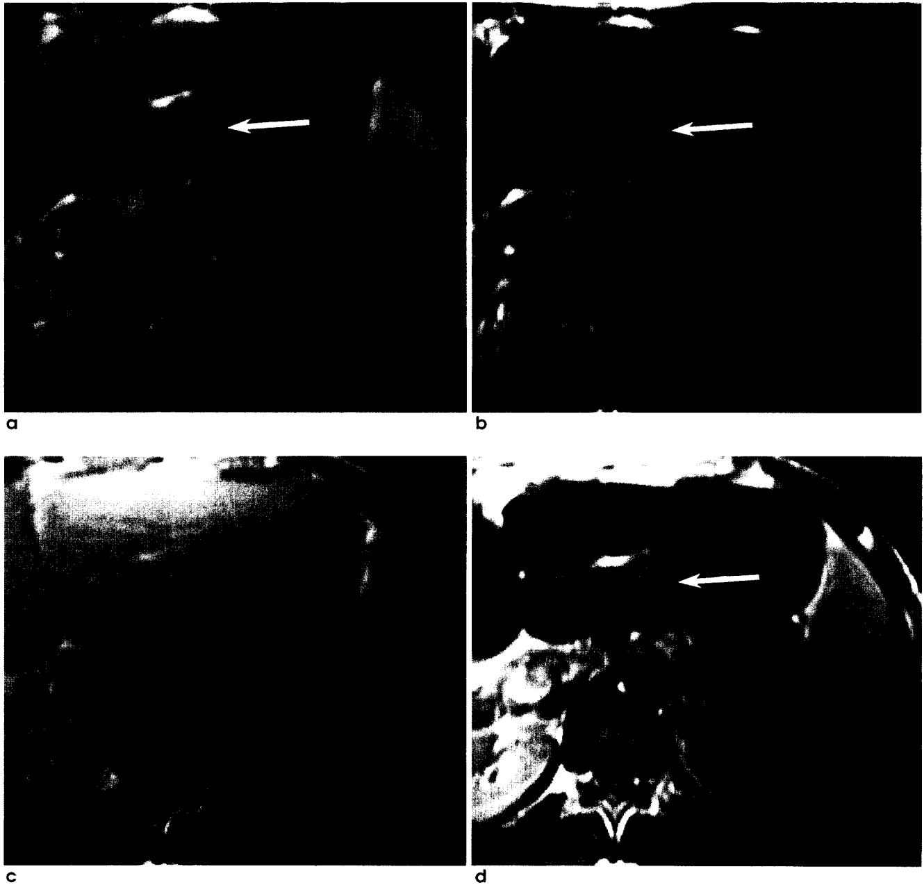
Fig. 4. Improved lesion-to-liver contrast of metastatic tumor with superparamagnetic iron oxide on T2-weighted and proton density weighted images. Precontrast T2-weighted spin echo (TR/TE = 2100msec/80msec) image shows a slightly high signal intensity nodule (arrow) in left lobe of the liver (a). Postcontrast T2-weighted spin echo (2100/80) image shows improved delineation of the lesion from decreased signal intensity of the liver parenchyma (b). Precontrast proton density weighted spin echo (2100/30) image shows poor liver-to-lesion contrast (c). Postcontrast proton density weighted image shows the best lesion-to-liver contrast (d).
