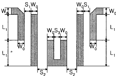
(d) Hybrid hairpin-line/half-wave parallel-coupled-line 여파기 (Hybrid(B))
