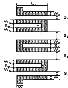
(b) Hairpin-line여파기
