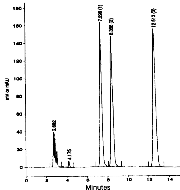
Fig. 1. Chromatogram of standard additives.
