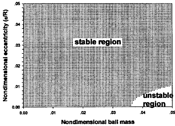
Fig. 6 Stability for \tilde{m} vs. \tilde{\epsilon} in the neighborhood of the equilibrium position corresponding to \tilde{r}_0 \neq 0 ( \tilde{\omega}=0.6 , \zeta=0.0707 and \beta=0.1168 ).
