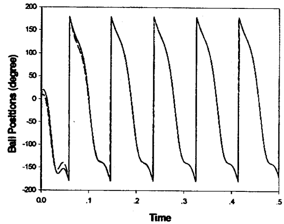
Fig. 12 Time history of \phi_1 and \phi_2 when the automatic ball balancer is not in the stable region corresponding to either \tilde{r}_0=0 or \tilde{r}_0 \neq 0 ( \tilde{\omega}=1 , n=2 , \tilde{m}=0.0328 , \zeta=0.0707 , \tilde{\varepsilon}=0.02 , \beta=0.1168 ).
