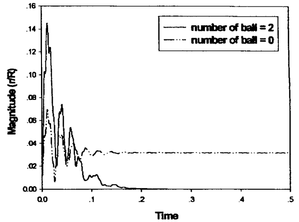
Fig. 7 Time history of \tilde{r} when the automatic ball balancer is in the stable region corresponding to \tilde{r}_0=0 ( \tilde{\omega}=1.6 , n=2 , \tilde{m}=0.0328 , \zeta=0.0707 , \tilde{\epsilon}=0.02 , \beta=0.1168 )
