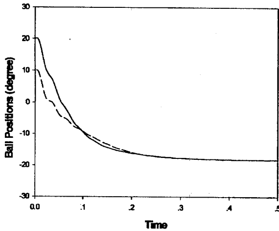
Fig. 10 Time history of \phi_1 and \phi_2 when the automatic ball balancer is in the stable region corresponding to \tilde{r}_0 \neq 0 ( \tilde{\omega}=0.6 , n=2 , \tilde{m}=0.0328 , \zeta=0.0707 , \tilde{\varepsilon}=0.02 , \beta=0.1168 )
