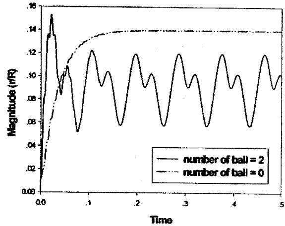
Fig. 11 Time history of \tilde{r} when the automatic ball balancer is not in the stable region corresponding to either \tilde{r}_0=0 or \tilde{r}_0 \neq 0 ( \tilde{\omega}=1 , n=2 , \tilde{m}=0.0328 , \zeta=0.0707 , \tilde{\varepsilon}=0.02 , \beta=0.1168 )
