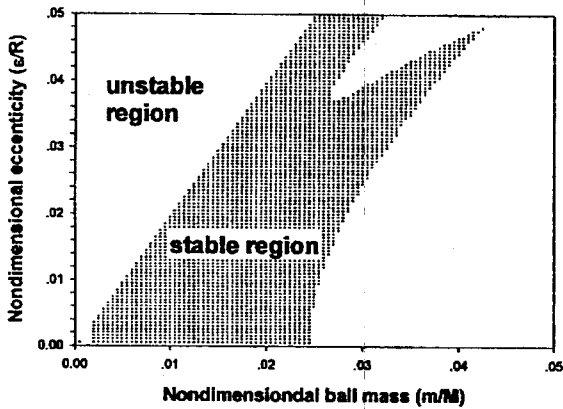
Fig. 4 Stability for \tilde{m} vs. \tilde{\epsilon} in the neighborhood of the equilibrium position, corresponding to \tilde{r}_0 = 0 ( \tilde{\epsilon} = 1.6 , \zeta = 0.0707 and \beta = 0.1168 )
