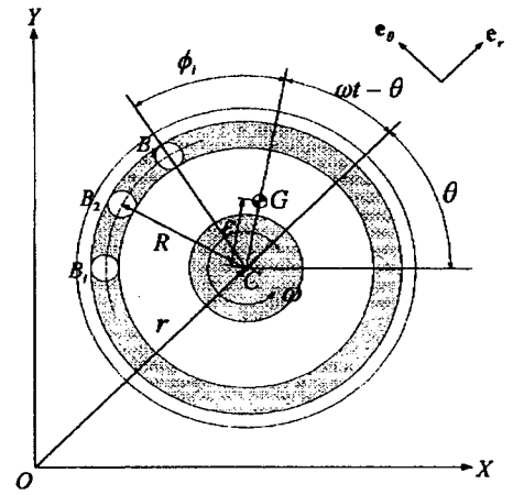
Fig. 2 Configuration of the automatic ball balancer
