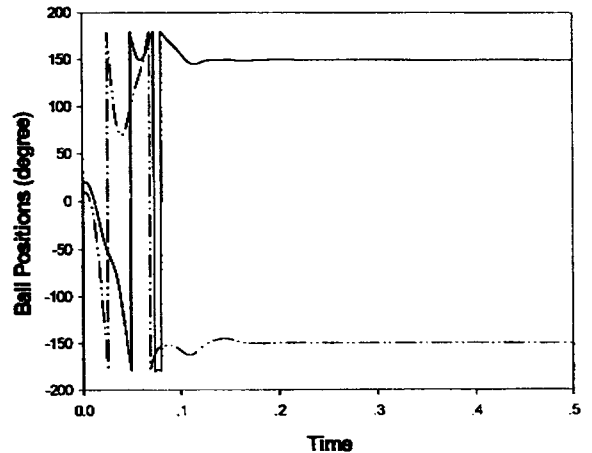
Fig. 8 Time history of \phi_1 and \phi_2 when the automatic ball balancer is in the stable region corresponding to \tilde{r}_0=0 ( \tilde{\omega}=1.6 , n=2 , \tilde{m}=0.0328 , \zeta=0.0707 , \tilde{\epsilon}=0.02 , \beta=0.1168 )
