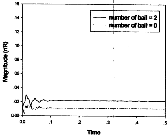
Fig. 9 Time history of \tilde{r} when the automatic ball balancer is in the stable region corresponding to \tilde{r}_0 \neq 0 ( \tilde{\omega}=0.6 , n=2 , \tilde{m}=0.0328 , \zeta=0.0707 , \tilde{\varepsilon}=0.02 , \beta=0.1168 )
