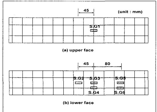
Fig. 3. Strain gage placements for stitched sandwich composite
