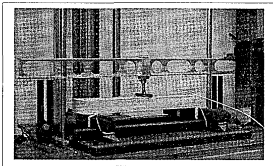
(b) Test fixture with stitched sandwich composite
