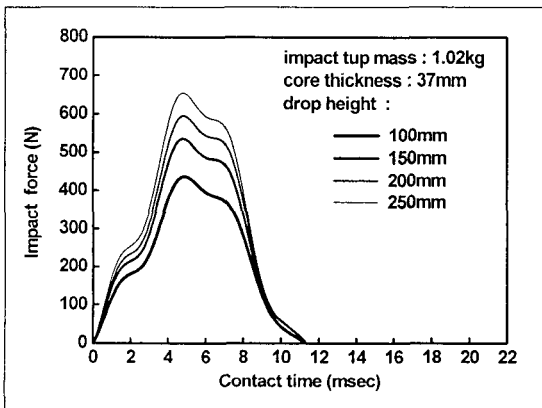
Fig. 5. Curves of impact force vs. contact time for various drop heights
