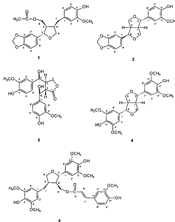
Fig. 1. Structures of compounds 1-5
