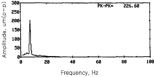
Fig. 8 Spectrum of shaft vibration (m=0.0)
