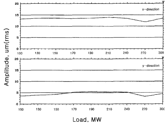
(a) Synchronous whirl component
