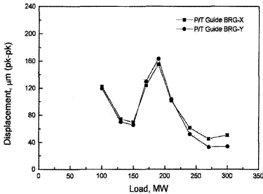
Fig. 6 Shaft vibration(overall) versus power load
