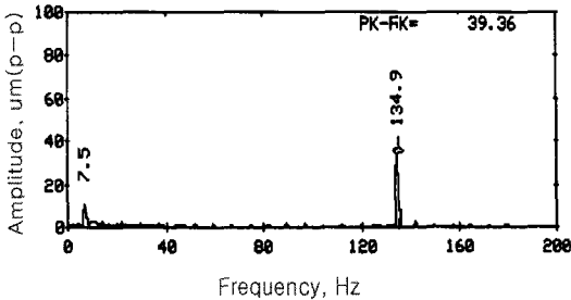
Fig. 9 Spectrum of shaft vibration (m=0.87)
