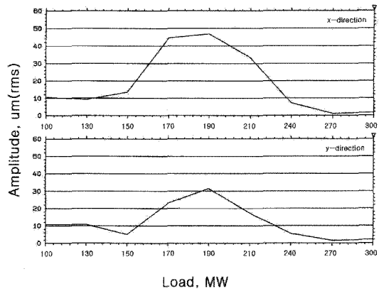
(b) Subsynchronous whirl component
