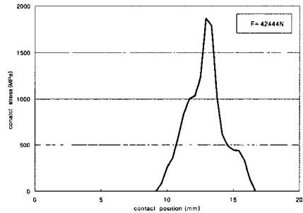
Fig. 4 Contact stress distribution in lateral direction.
