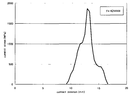
(a) 3-D F.E. analysis
