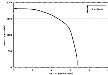
Fig. 5 Contact stress distribution in longitudinal direction.
