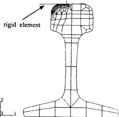
Fig. 7 Finite element mesh for optimization design.
