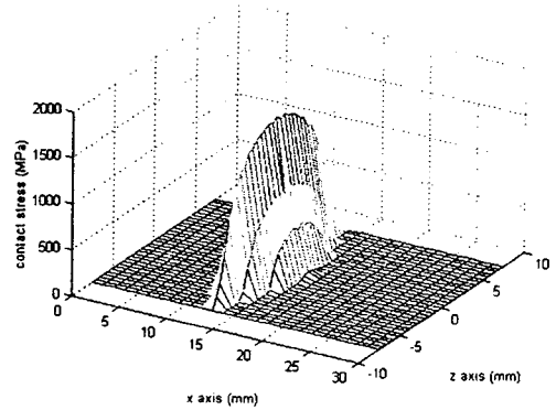
Fig. 3 Contact stress distribution of wheel-rail.
