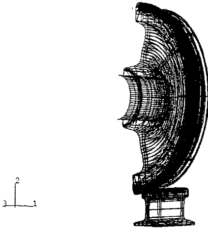
Fig. 2 Finite element mesh for wheel-rail contact.
