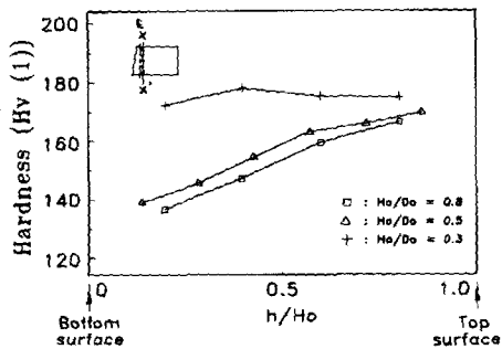
Fig. 8 Distributions of hardness for different aspect ratio (pure iron)
