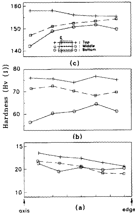
Fig. 7 Variation of hardness in (a) preform (b) resinted sample (c) rotary forging sample (pure iron)
