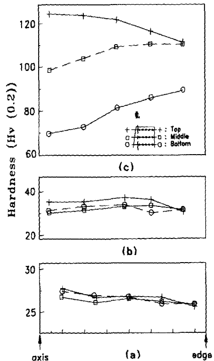
Fig. 10 Variation of hardness in (a) preform (b) resinted sample (c) rotary forging sample (pure copper)
