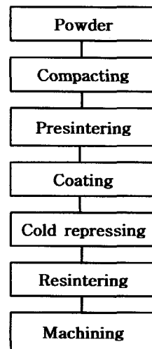
Fig. 1 Cold rotary repressing process
